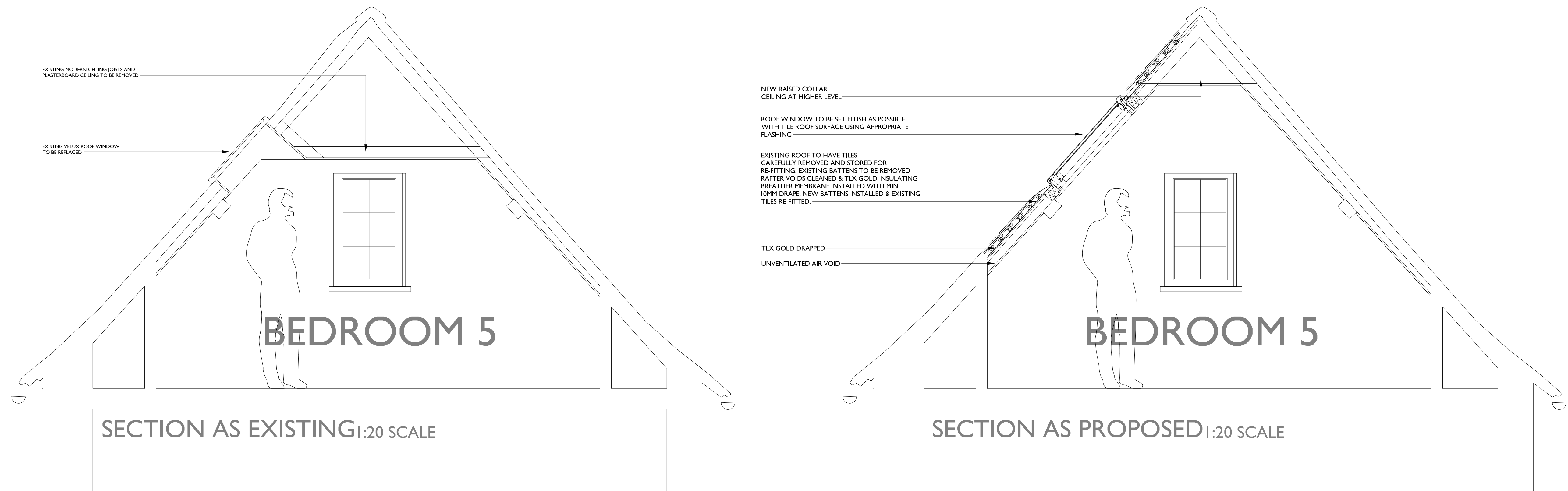
BEDROOM 5 CEILING ALTERATIONS & ROOF INSULATION DETAILS
