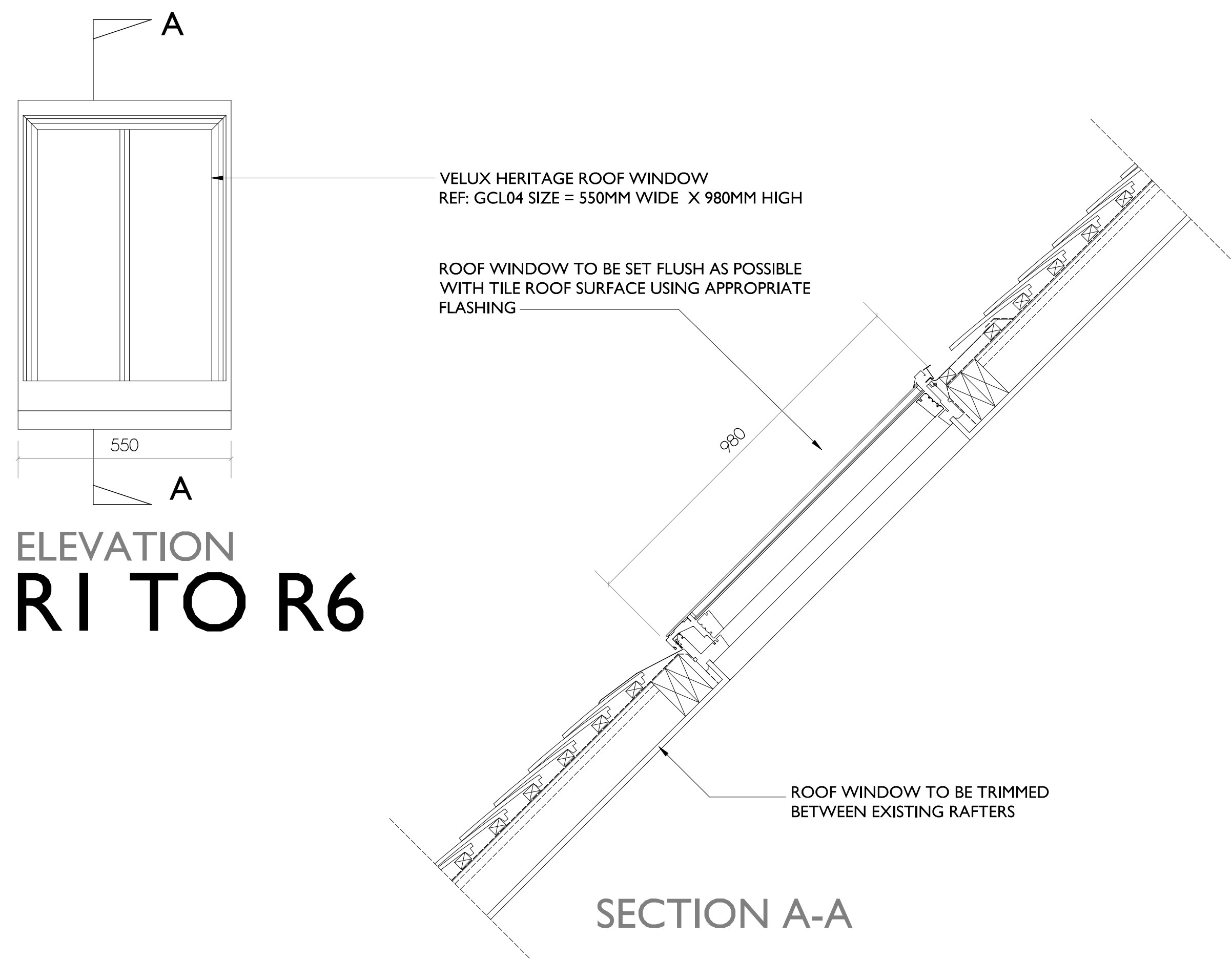
NEW ROOF WINDOW DETAILS 1:10 SCALE
