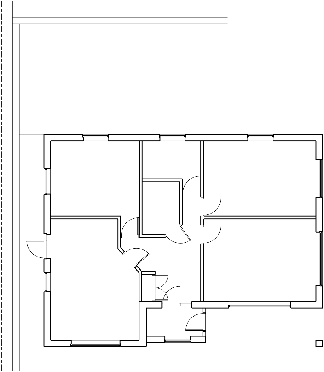
EXISTING PLAN
