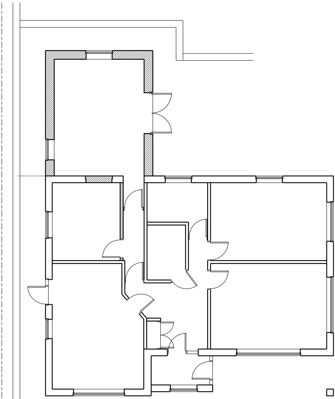
PROPOSED PLAN
