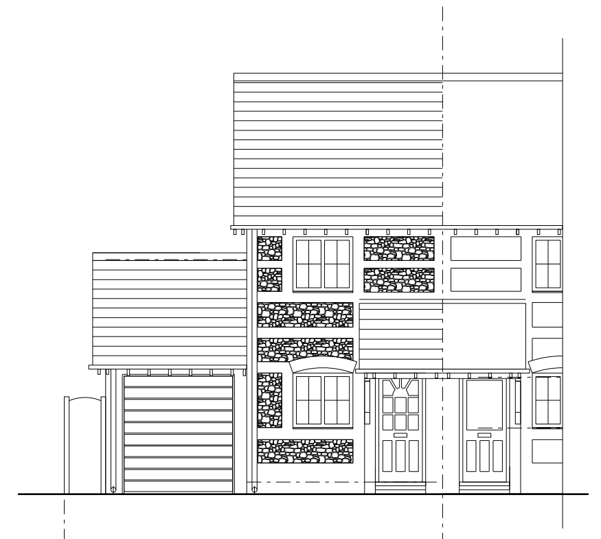
South Elevation 1:100
