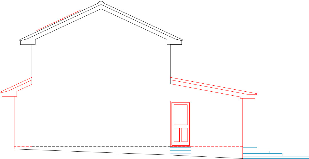
West Elevation
