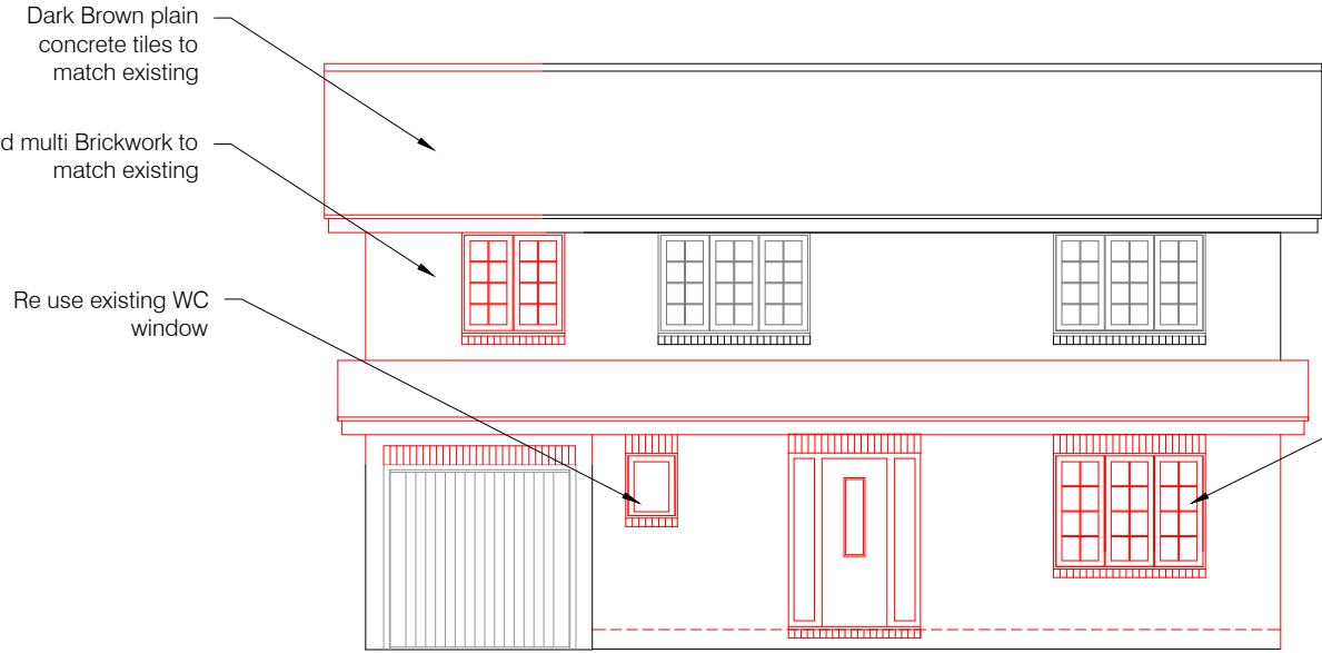
North Elevation
