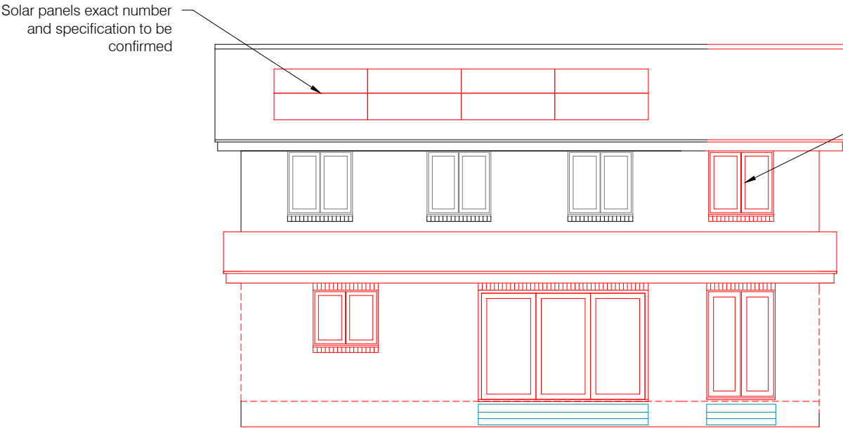
South Elevation
