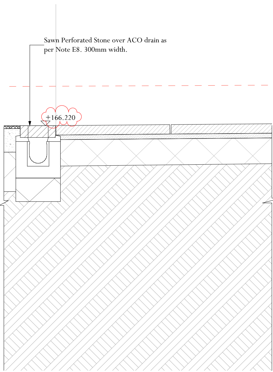
C-C Forecourt, Detail 2 1:20
