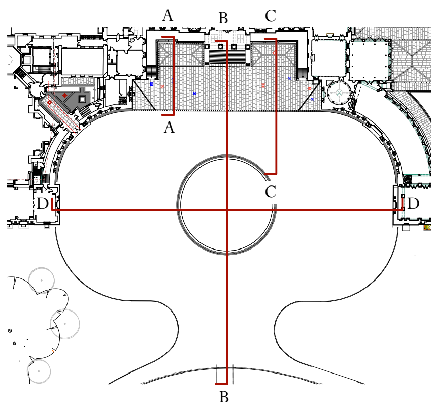
Forecourt Key Plan 1:1000
