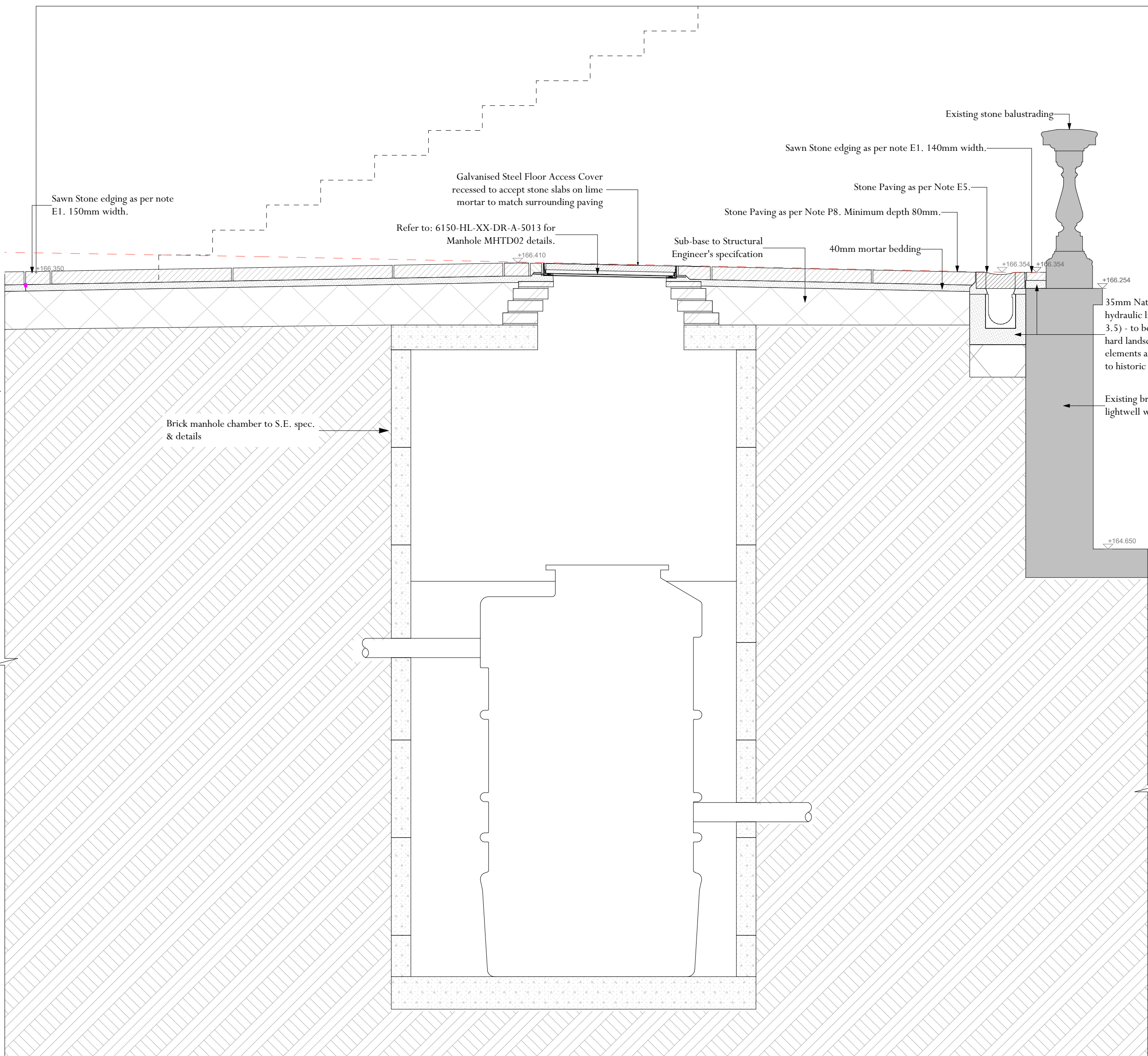
C-C Forecourt, Detail 3
