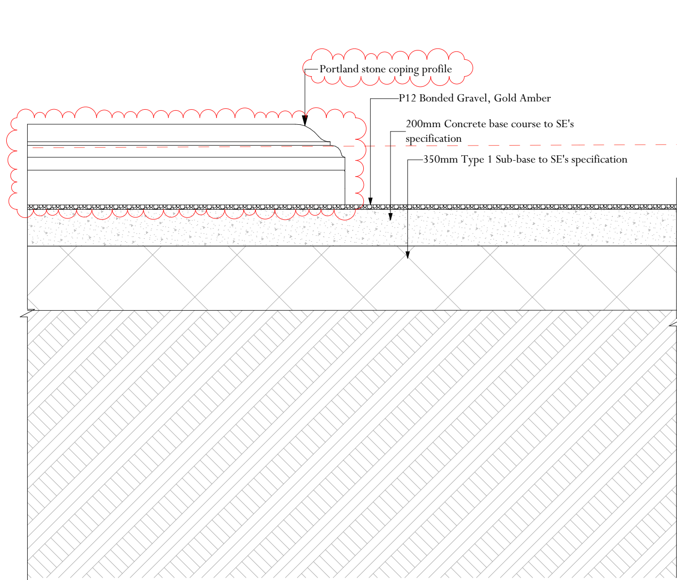
C-C Forecourt, Detail 1 1:20
