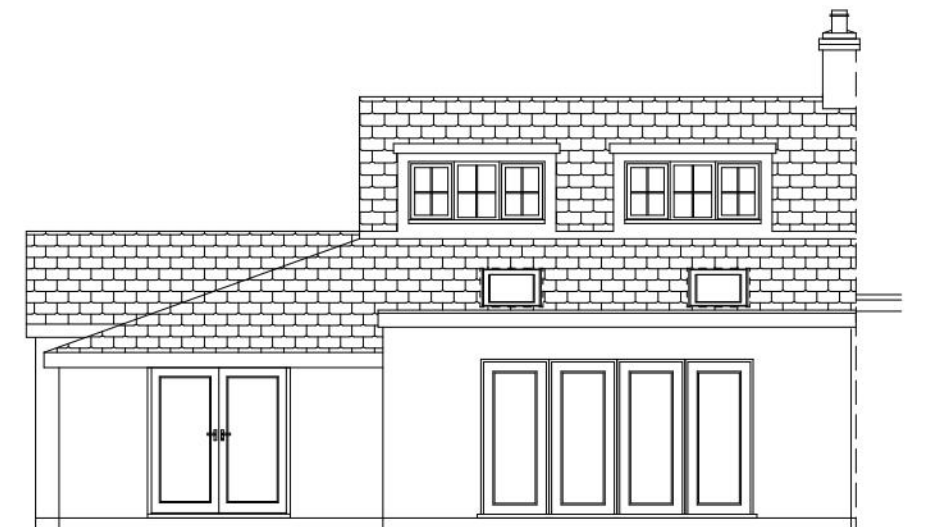
Proposed Rear
