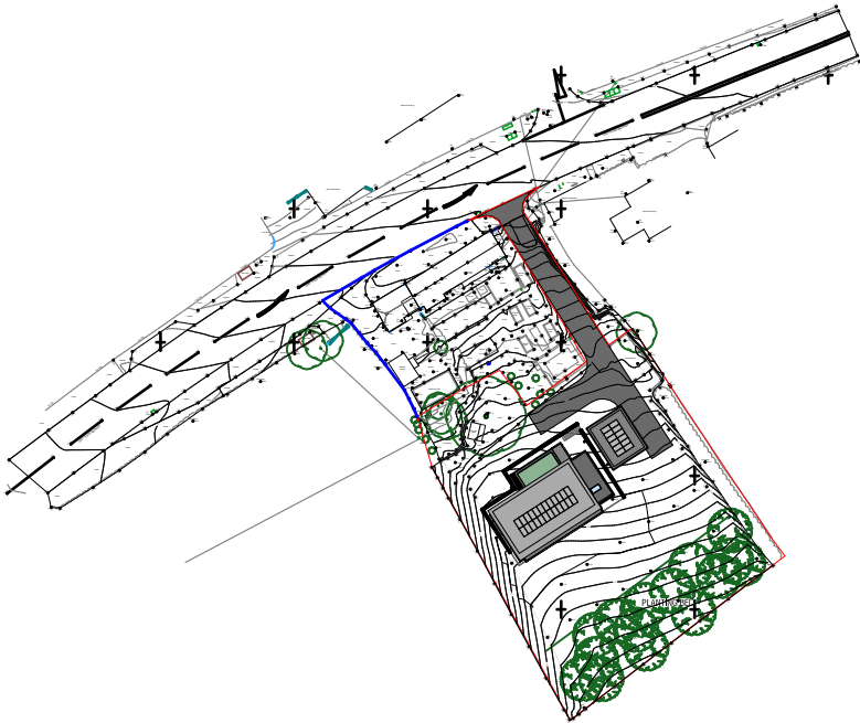
LOCATION PLAN 1:1250
