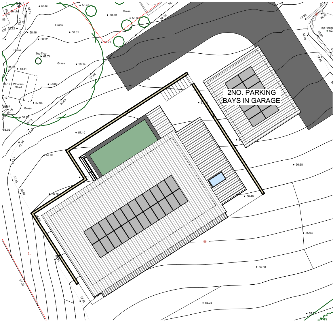
BLOCK PLAN 1:200
