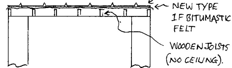
SECTION THROUGH ROOF
