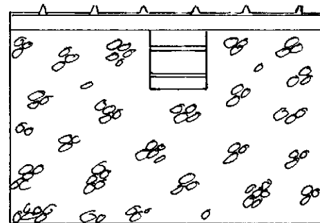
NW ELEVATION SHOWING NEW HORIZONTAL METAL BARS @ 30cm INTERVALS IN EXISTING OPENING
