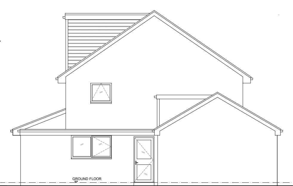
SIDE ELEVATION 2 POST LOFT CONVERSION (AS EXISTING)
