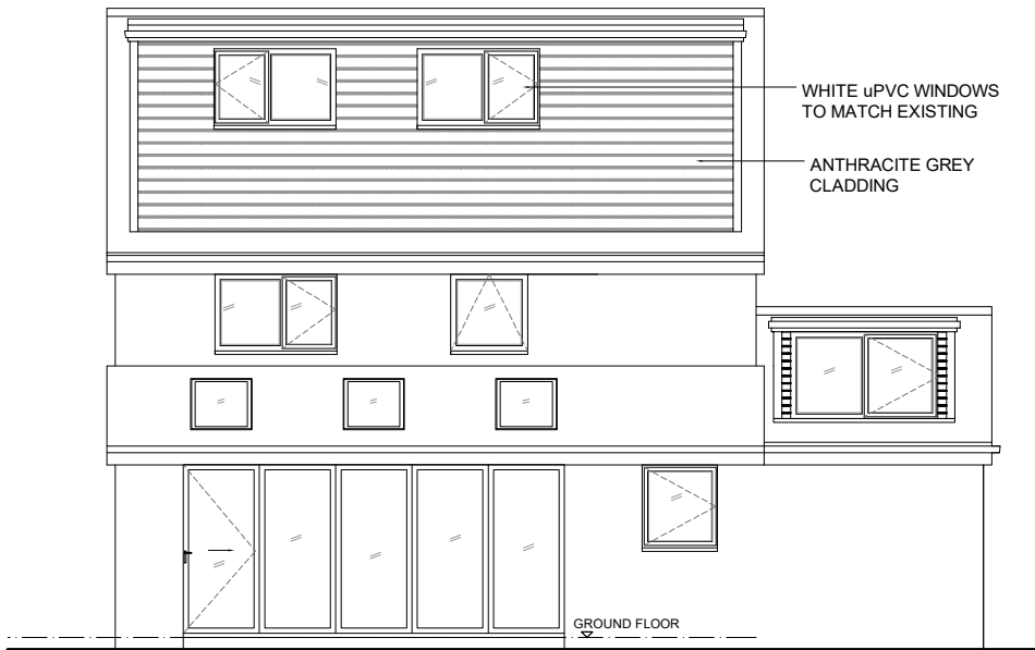
REAR ELEVATION POST LOFT CONVERSION (AS EXISTING)
