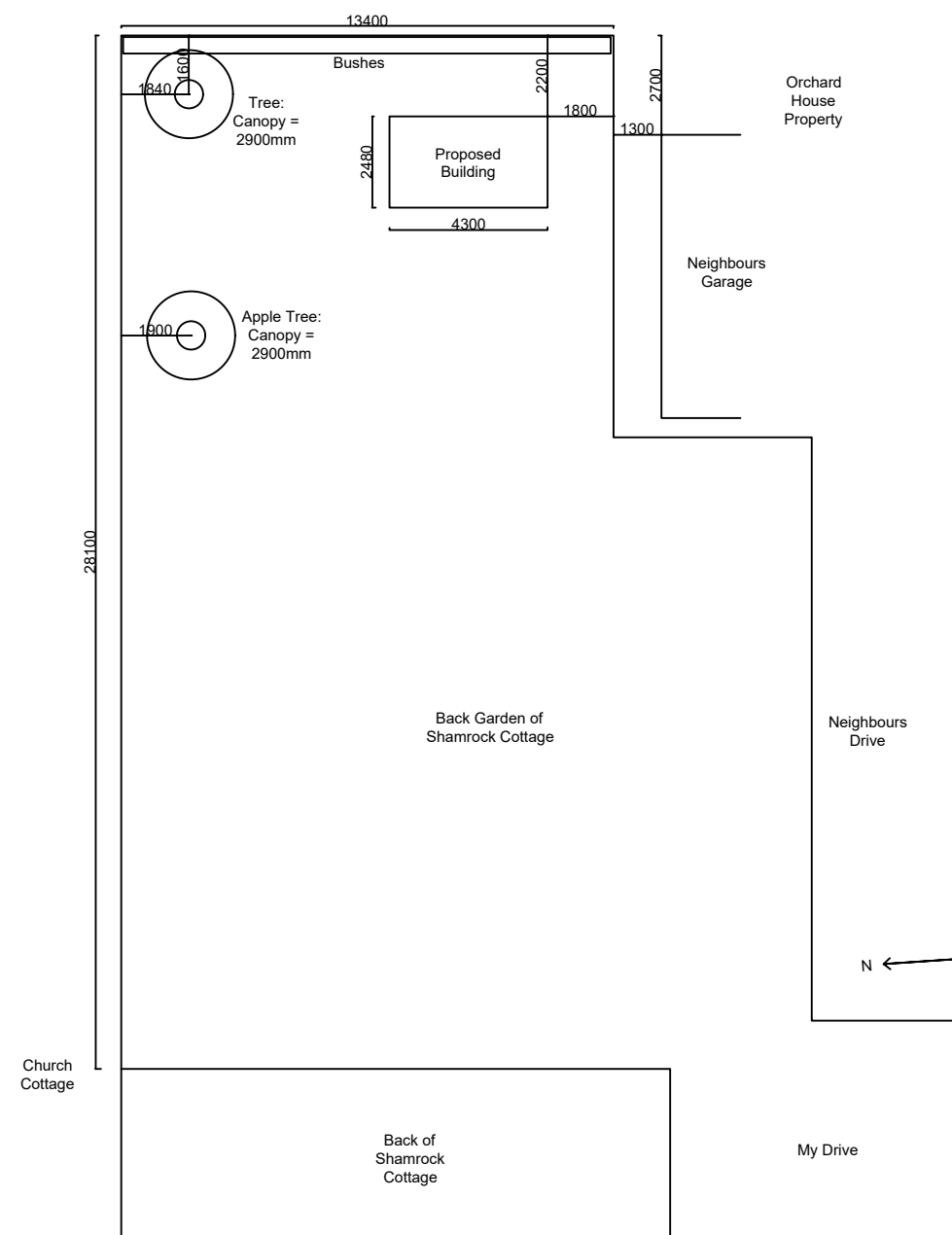
Proposed Site Layout (1:200)
