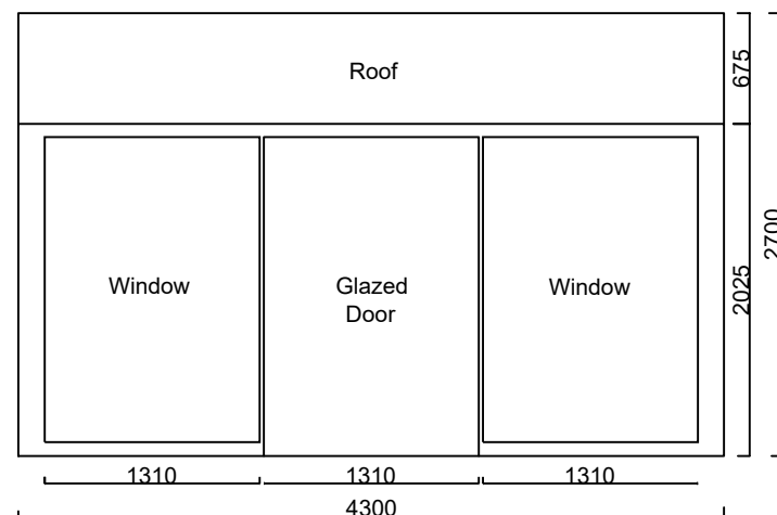
Proposed Front Elevation (1:50)
