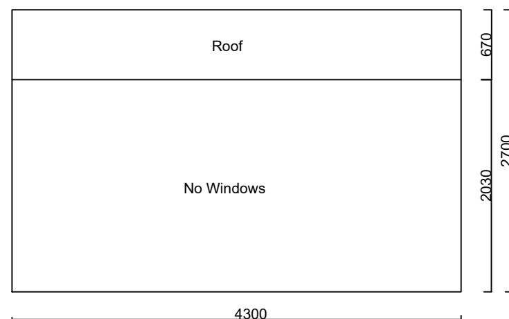
Proposed Rear Elevation (1:50)
