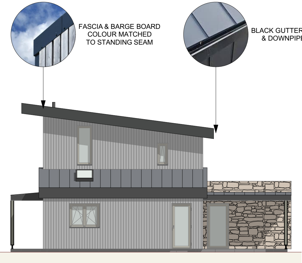
ELEVATION 4/NORTH EAST
