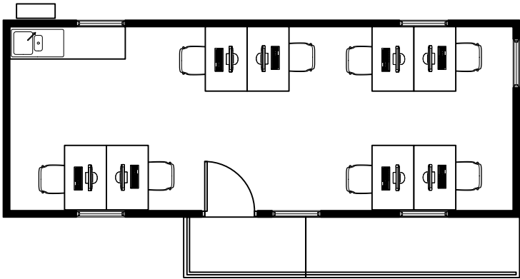
1/100 - Floor plan
