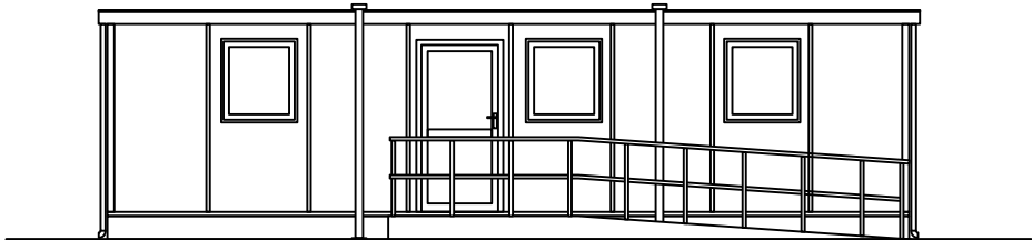
1/100 - Proposed NW (Front) elevation
