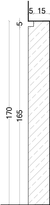
Detail 07 - First Floor marble
