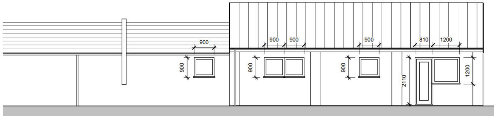
5 | North Elevation - Dimensions 1 : 100
