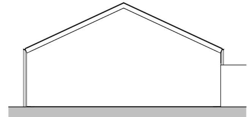
6 | West Elevation - Dimensions 1 : 100
