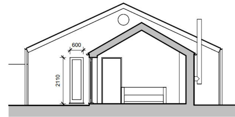
3 | East Elevation - Dimensions 1 : 100
