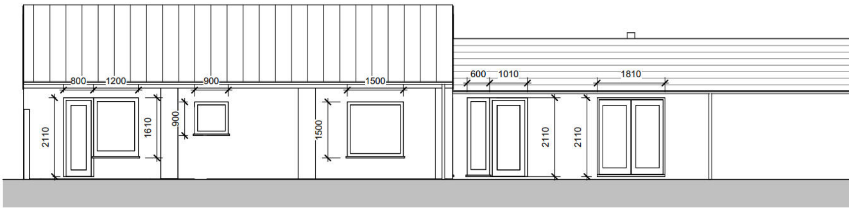
4 | South Elevation - Dimensions 1 : 100
