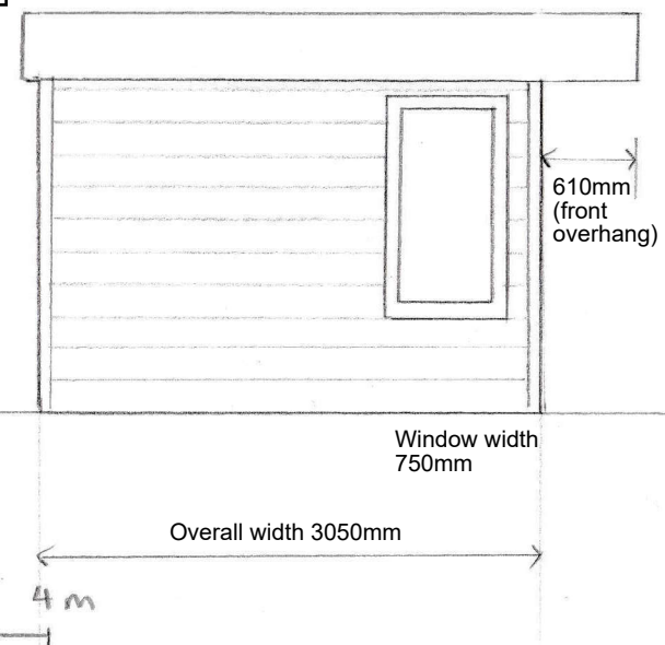
North elevation (side)
