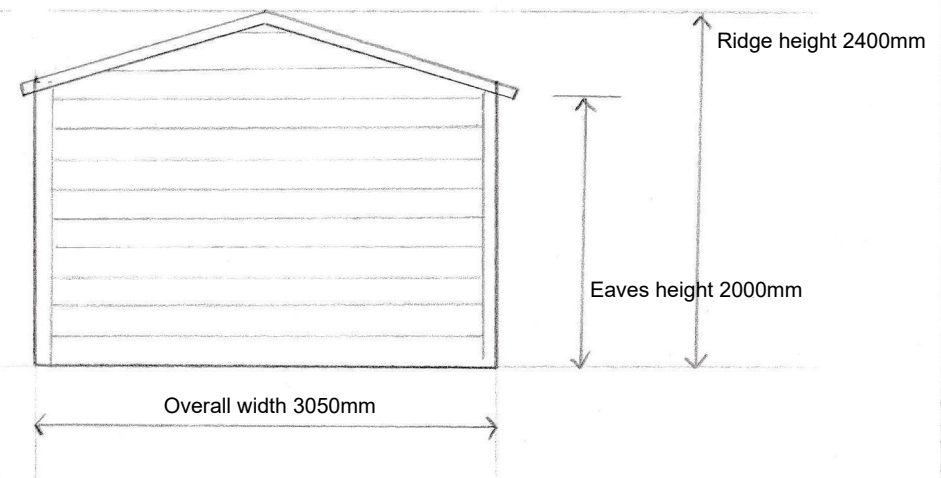
East elevation (rear of summer house)
