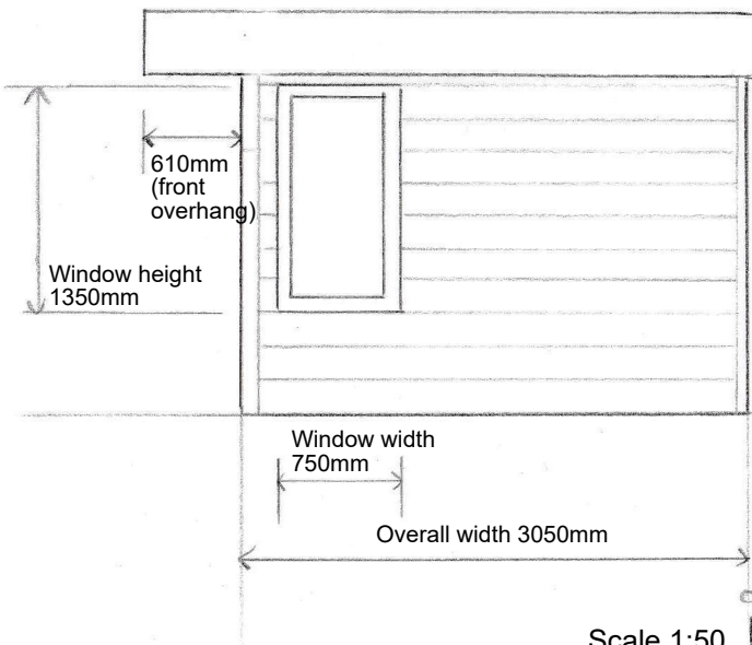
South elevation (side)
