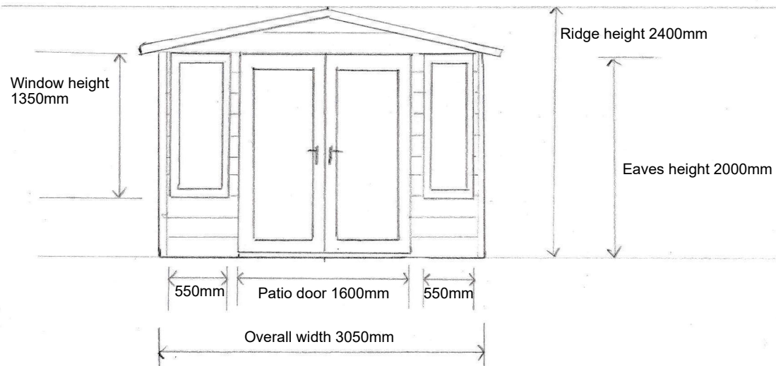
West elevation (front of summer house)
