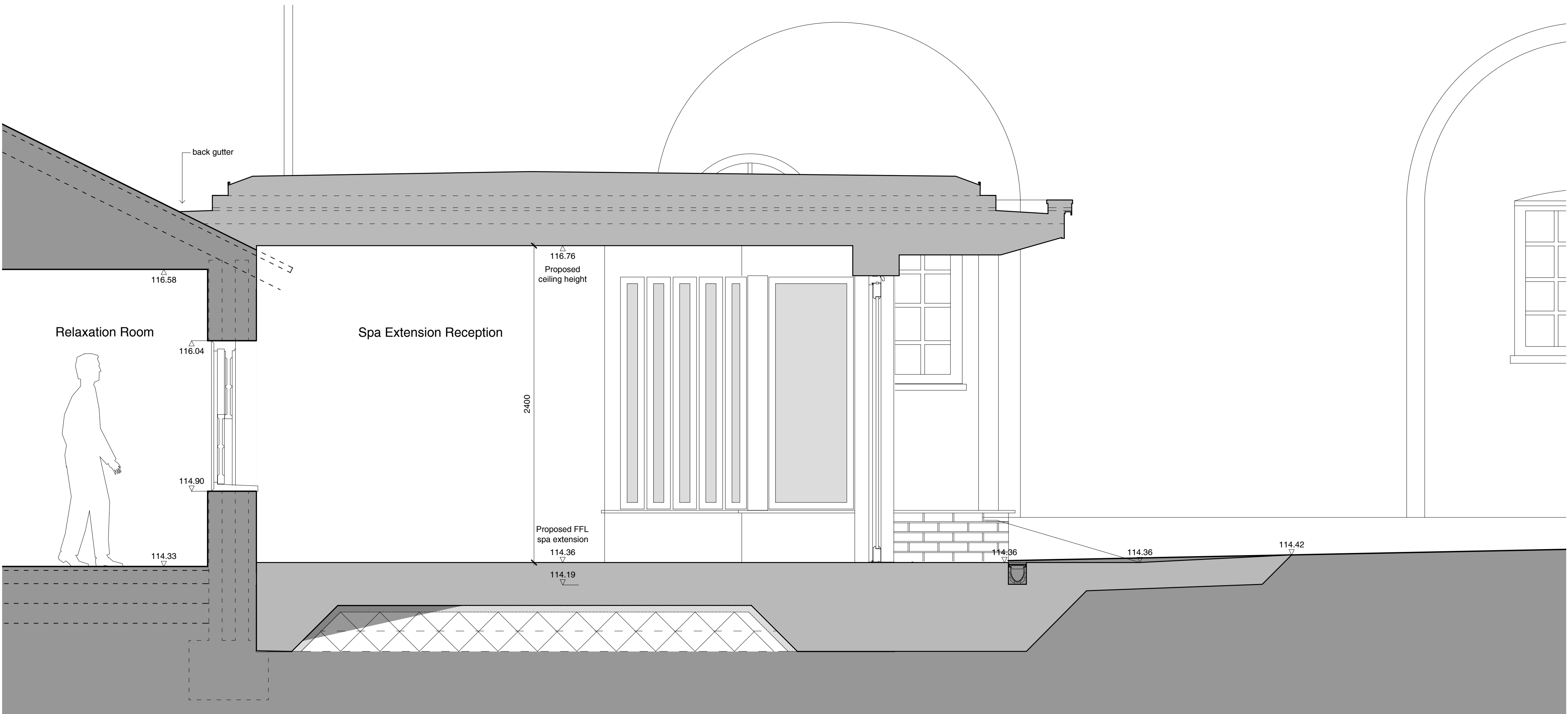
Section B-B as Proposed - 1:20
