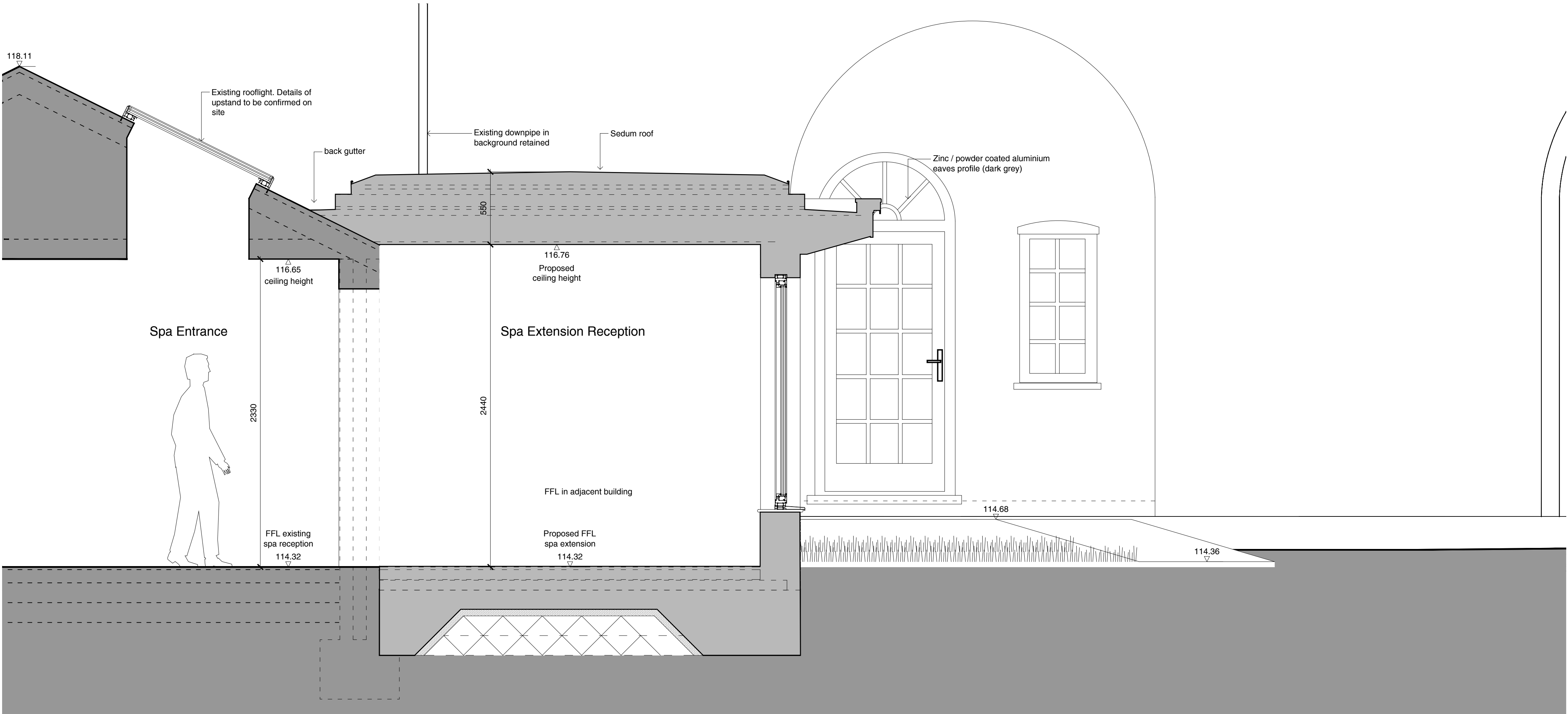
Section A-A as Proposed - 1:20
