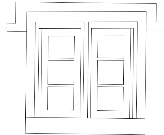
W-001.2 1:20 Existing Stone hood-moulding, surround and mullion, with white painted timber fixed casements. Casements to be replaced with double glazed white painted timber frames where muntin placements will match original. Stone elements to be retained and unimpacted by works.
