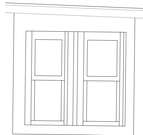
W-102.1 1:20 Existing Stone surround, lintel, and mullion, with white painted timber sash windows. Timber windows to be replaced with double glazed white painted timber frames. Stone elements to be retained and unimpacted by works.
