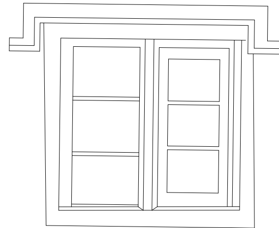
W-001.1 1:20 Existing Stone hood-moulding, surround and mullion, with white painted timber fixed casement (left) and white painted timber outward opening casement (right). Casements to be replaced with double glazed white painted timber frames where muntin placements will match original. Stone elements to be retained and unimpacted by works.
