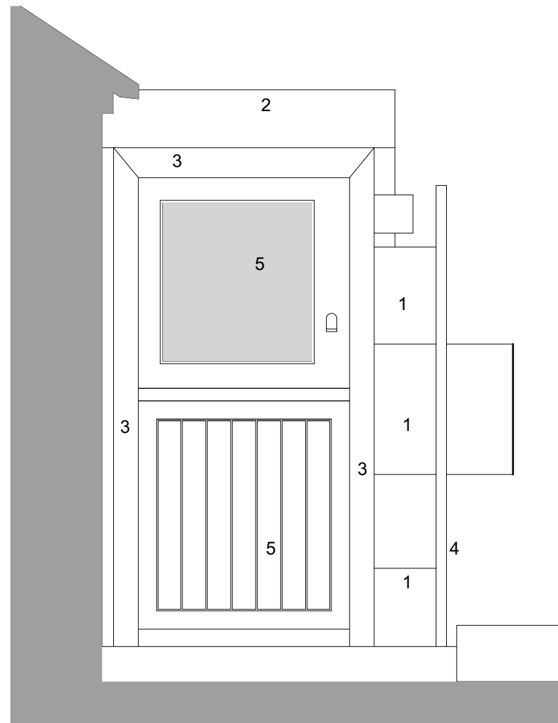
D-006.1 as Existing @ 1:20
