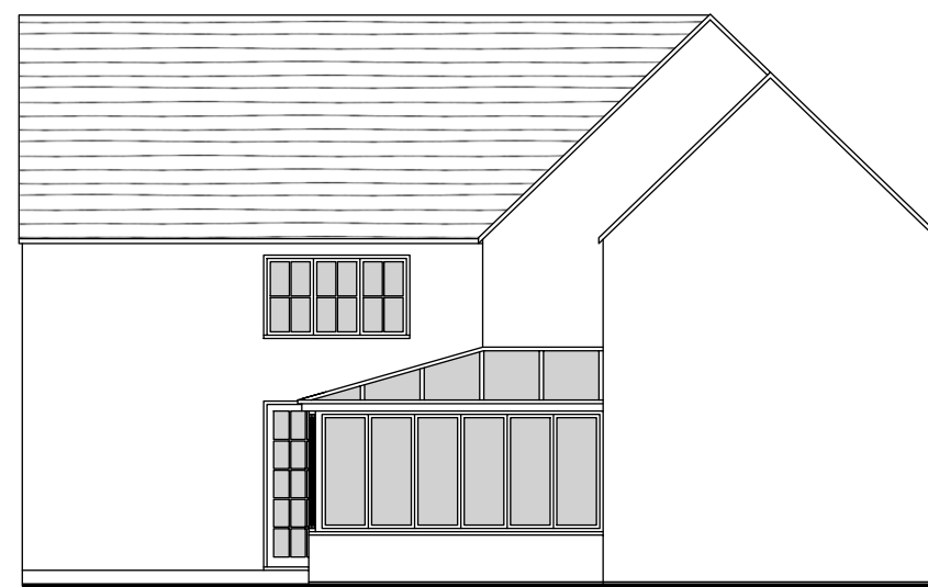
NORTH ELEVATION
