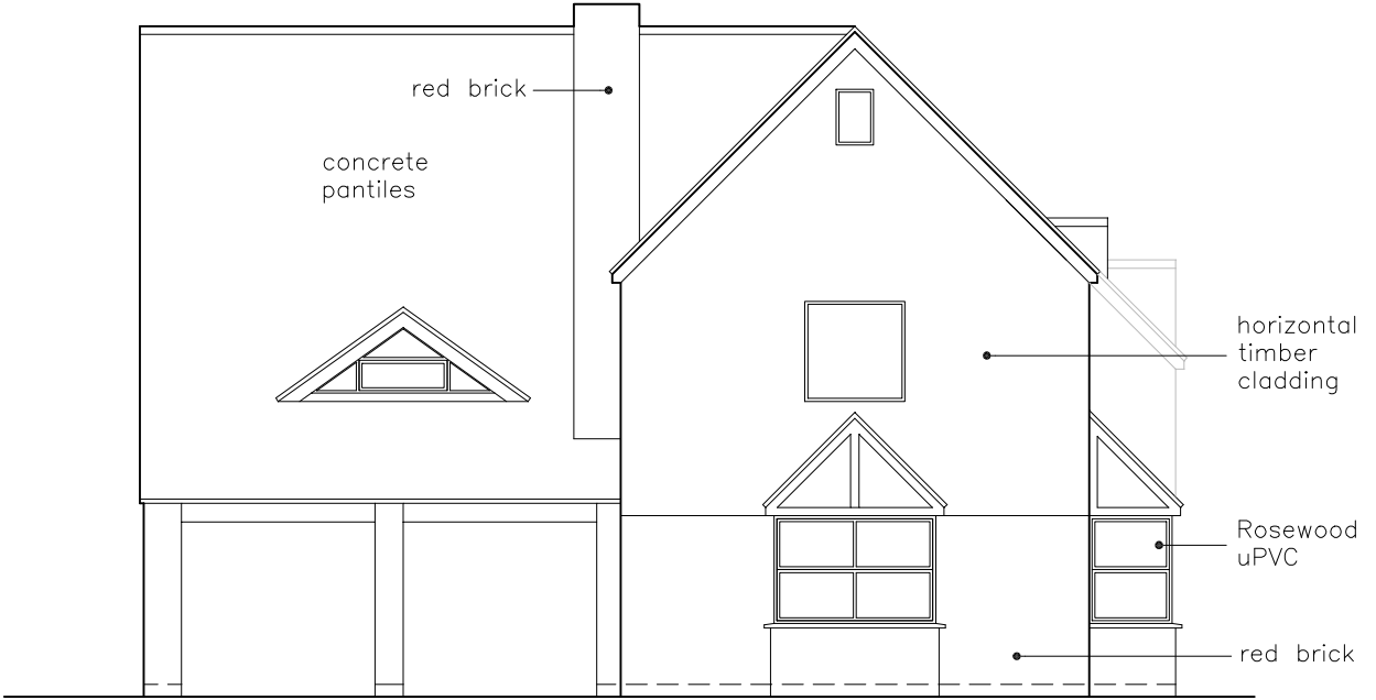
FRONT (N) ELEVATION
