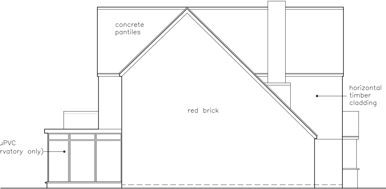
SIDE (E) ELEVATION
