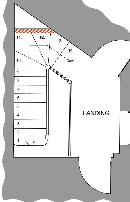
PROPOSED FIRST FLOOR STAIR LAYOUT (above hallway) Scale 1:50
