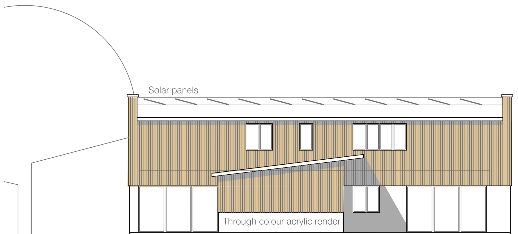
West Elevation
