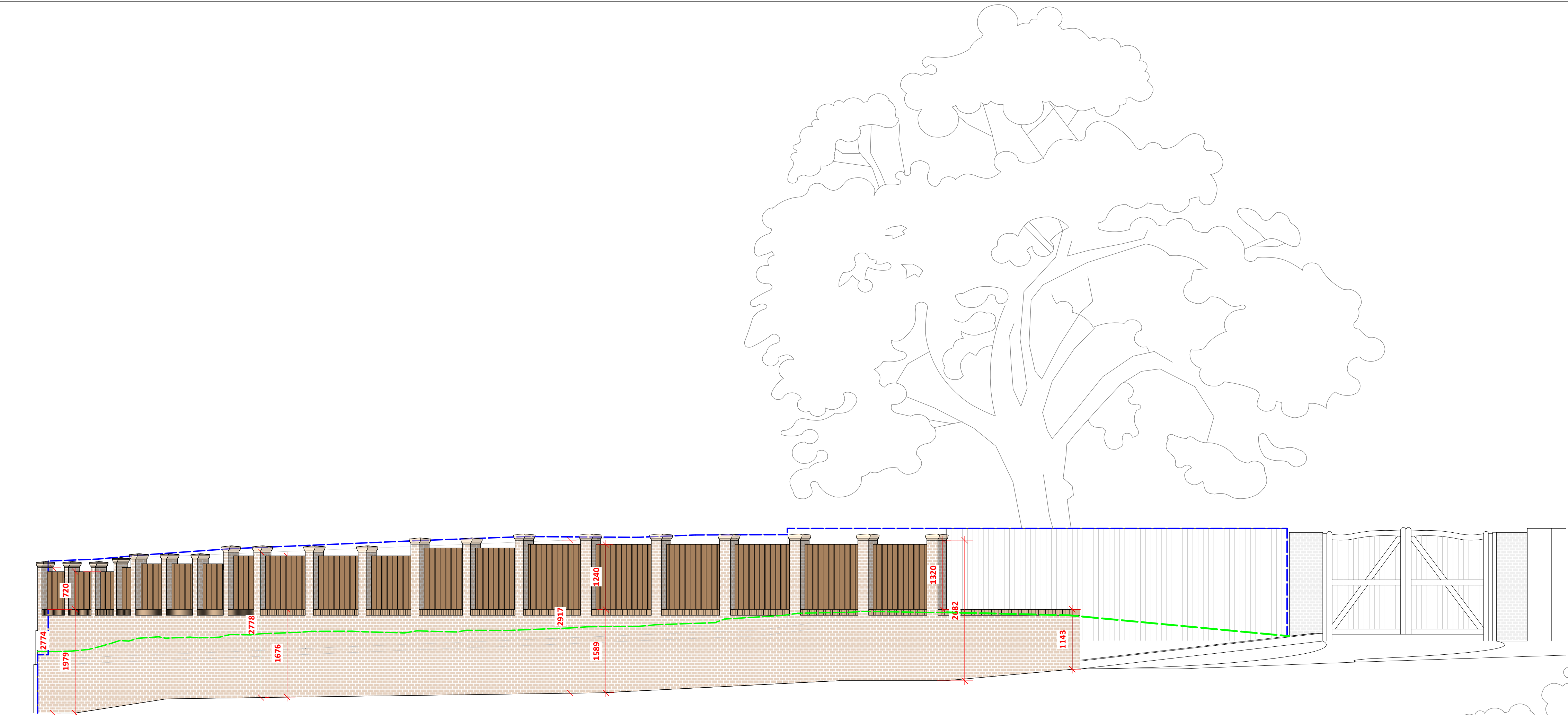
ELV PROPOSED N ELEVATION 01 1:50
