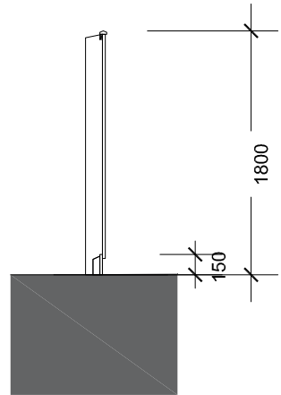
1800mm close board timber fence Elevation C
