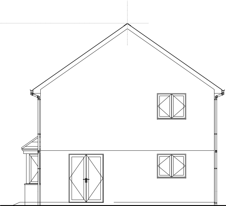
SIDE ELEVATION
