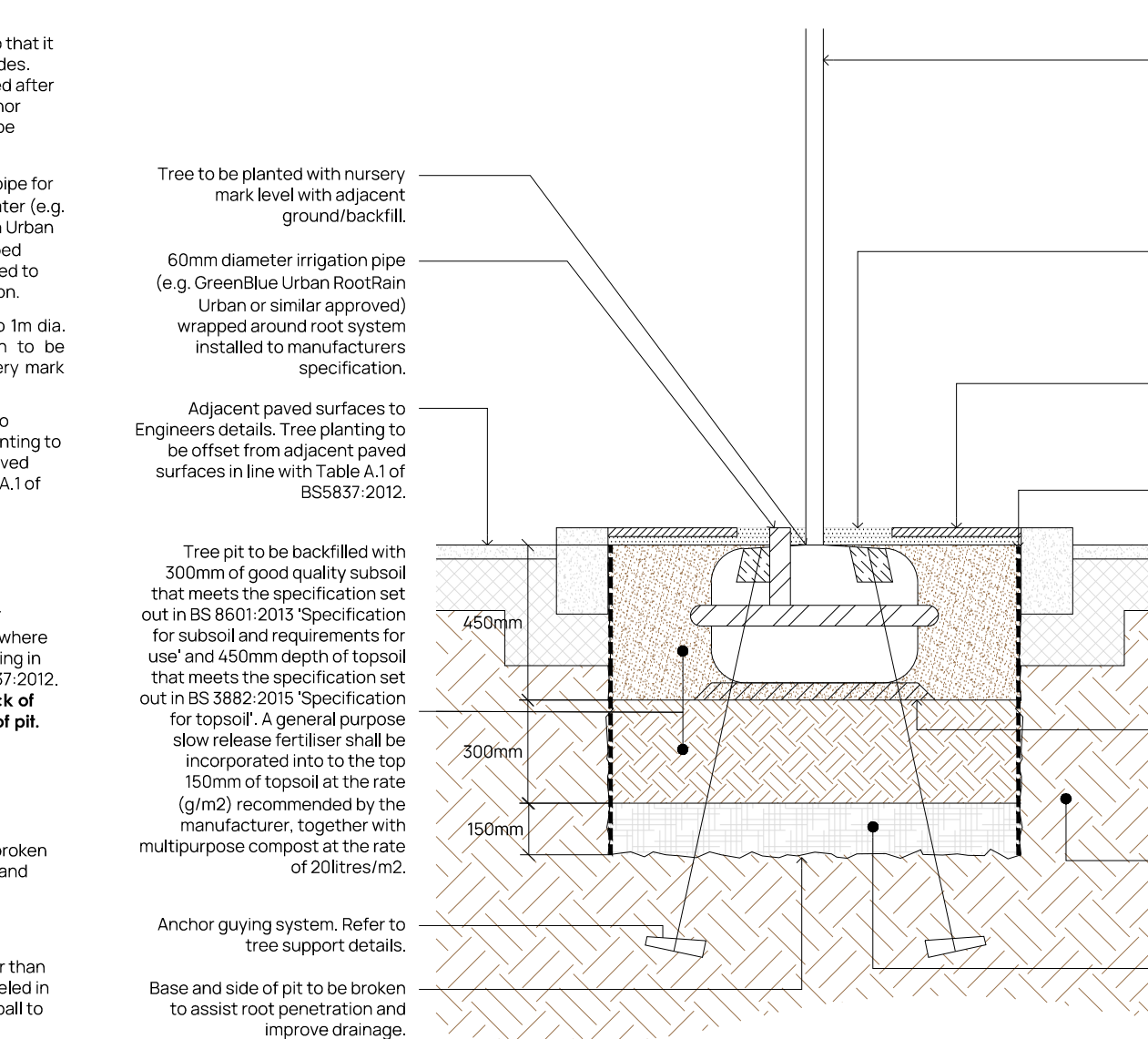
Detail 10 - Typical Tree Pit within Hard Landscape (N.T.S.)
