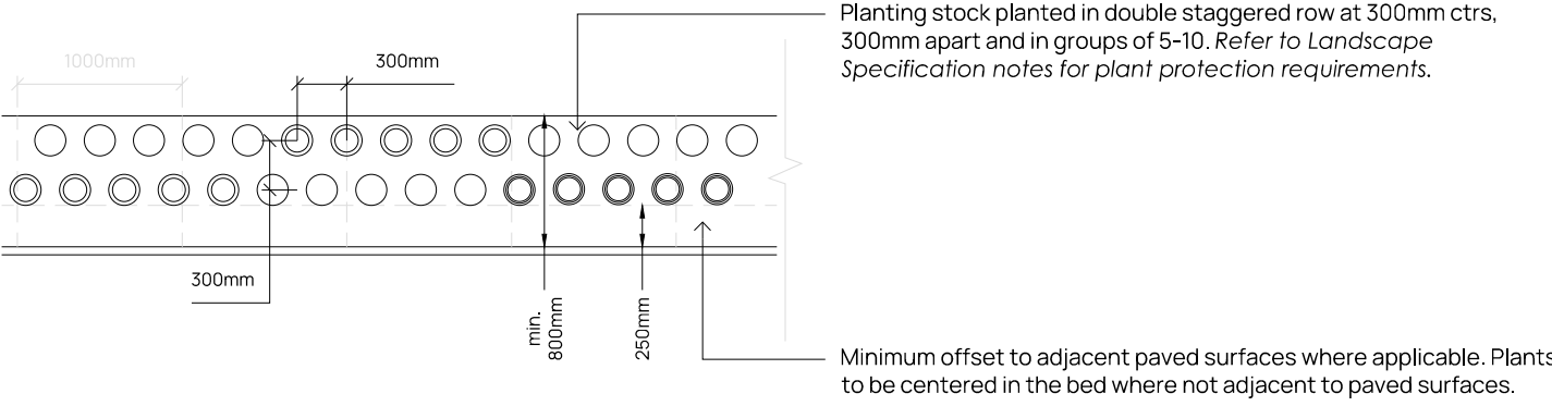
Detail 3 - Typical Native Hedgerow Double Staggered Layout (N.T.S.)
