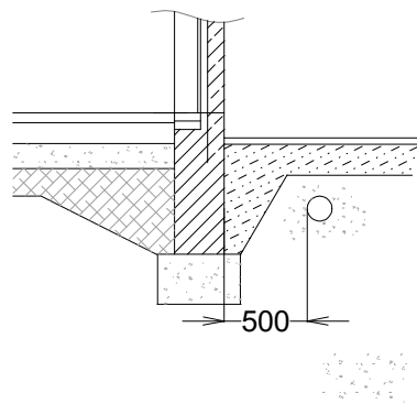
SECTION C-C
