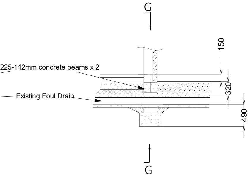
Typical drain section
