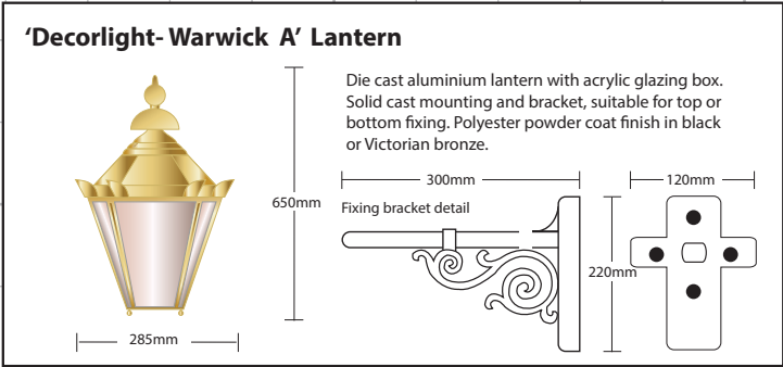
G TWO X LANTERNS FINISHED BRASS. SIZE. 0.28m x 650mm. H.A.G. 2.15m.
