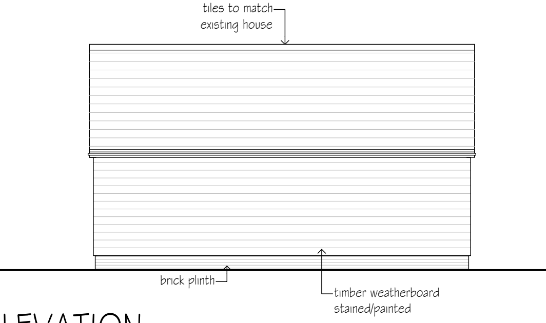
NORTH ELEVATION
