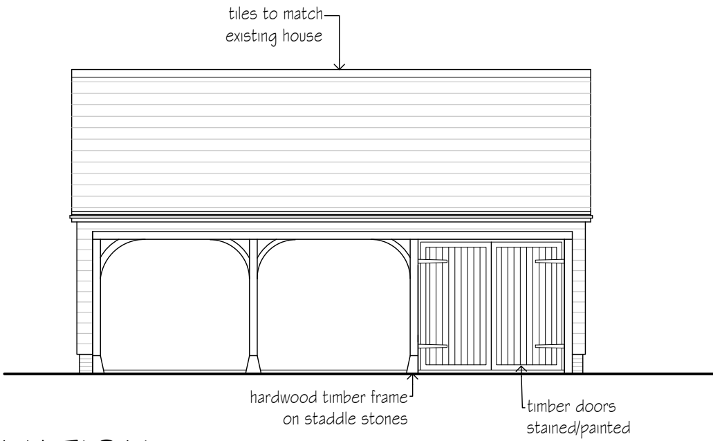
SOUTH ELEVATION
