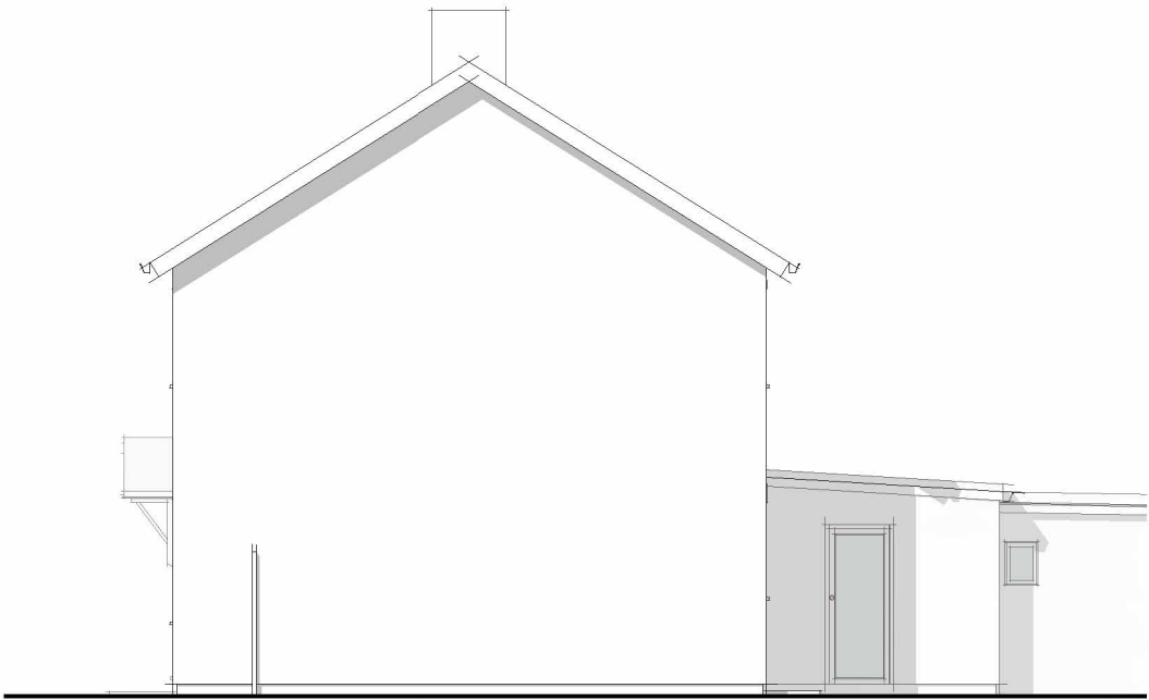
2 Existing Side (East) Elevation 1 : 100
