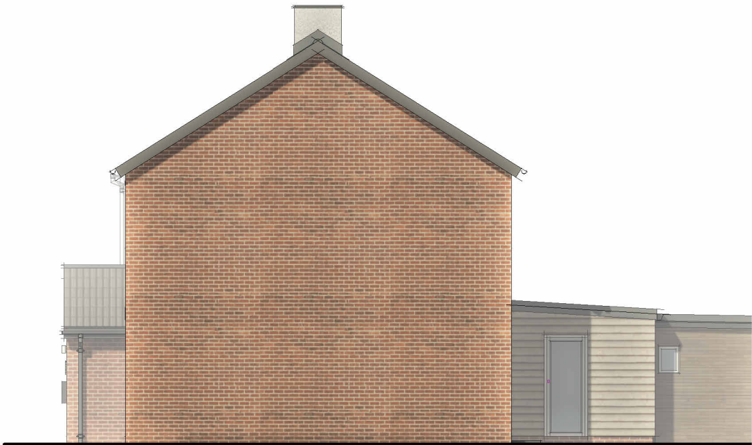
2 Proposed Side (East) Elevation 1 : 100
