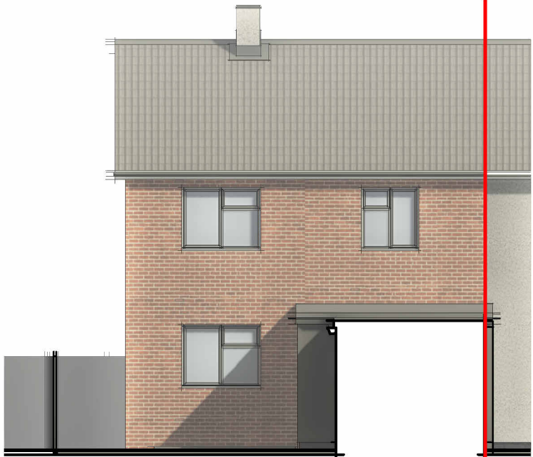
3 Proposed Rear (North) Elevation 1 : 100
