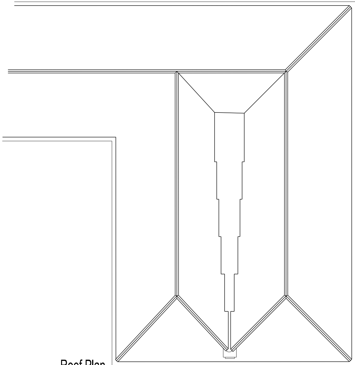
Roof Plan
