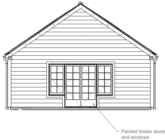
South Elevation
