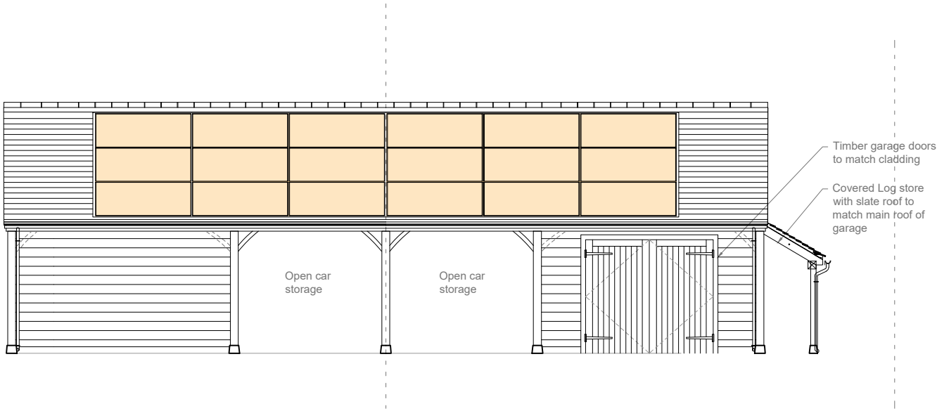
East Elevation
