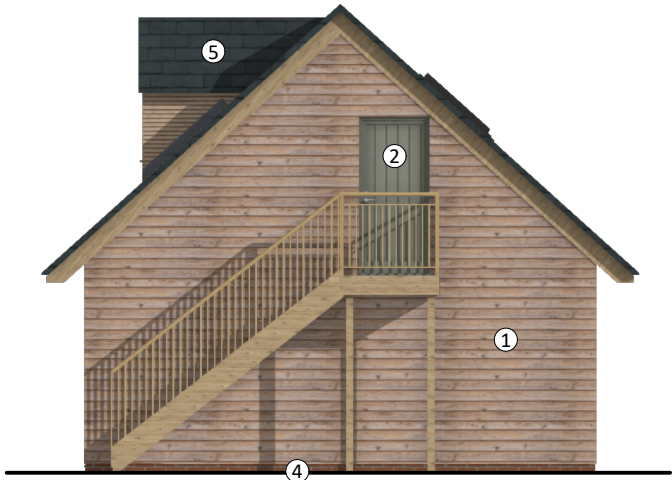
PROP. NORTH-EAST ELEVATION 1:100
