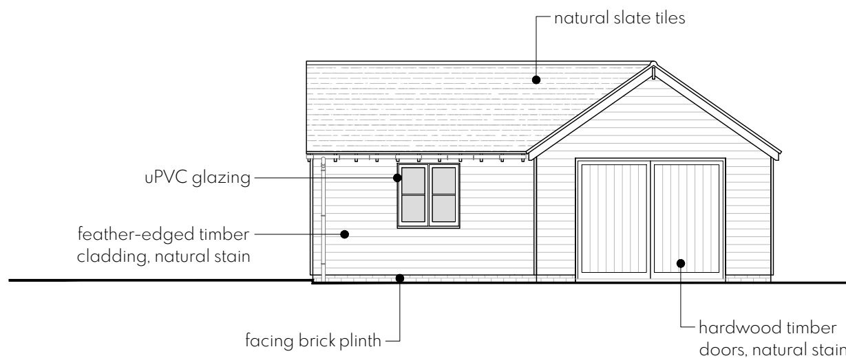
NW ELEVATION 1:100
