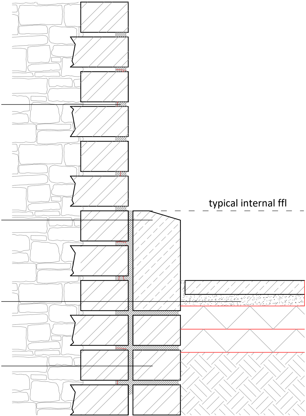
PROPOSED WALL PLINTH DETAIL
