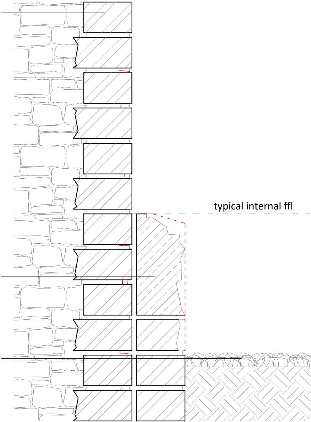
EXISTING WALL PLINTH DETAIL
