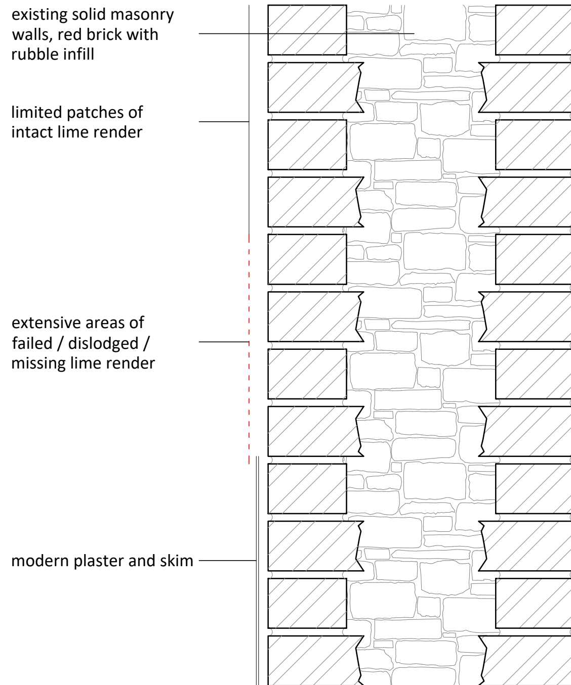
EXISTING WALL DETAIL
