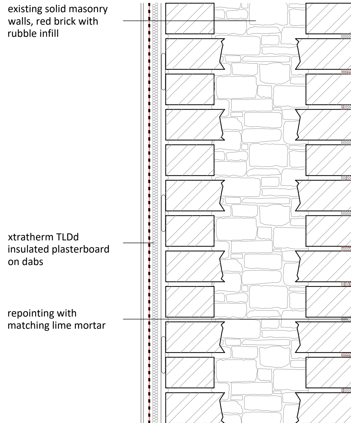
PROPOSED WALL DETAIL
