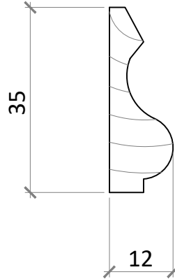
Picture Rail
