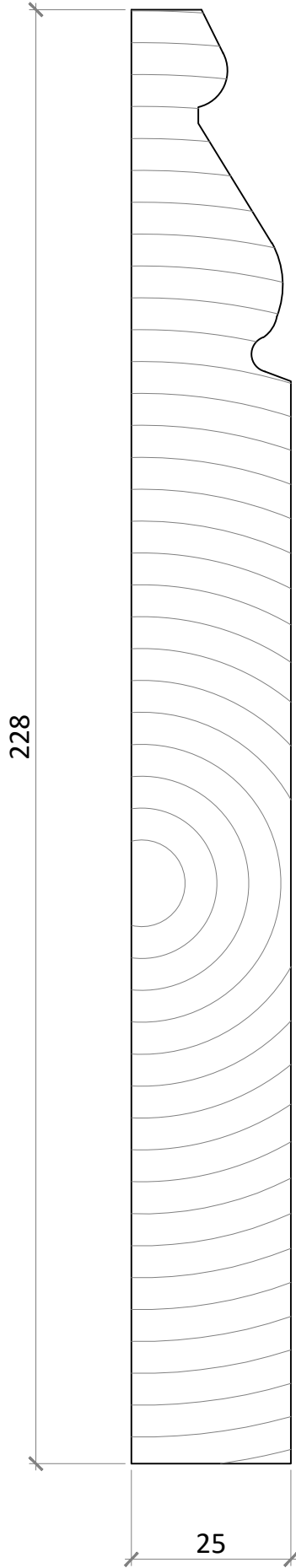
Skirting
