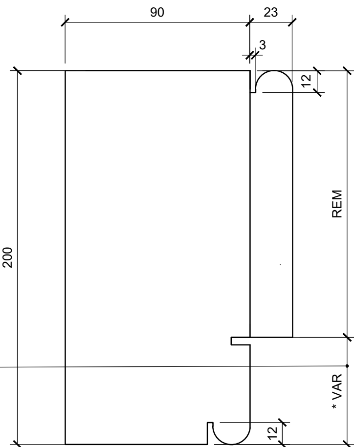
03 TYPICAL DOOR FRAME 1.2 @ A1 / 1:4 @ A3
