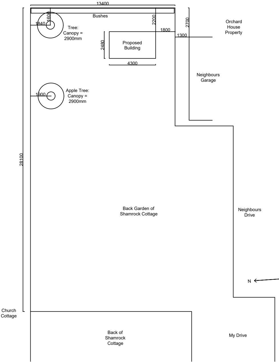
Proposed Site Layout (1:200)
