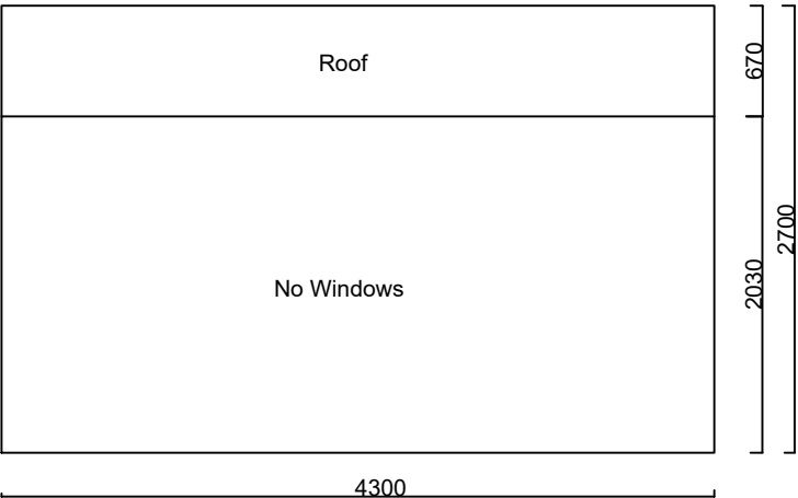
Proposed Rear Elevation (1:50)
