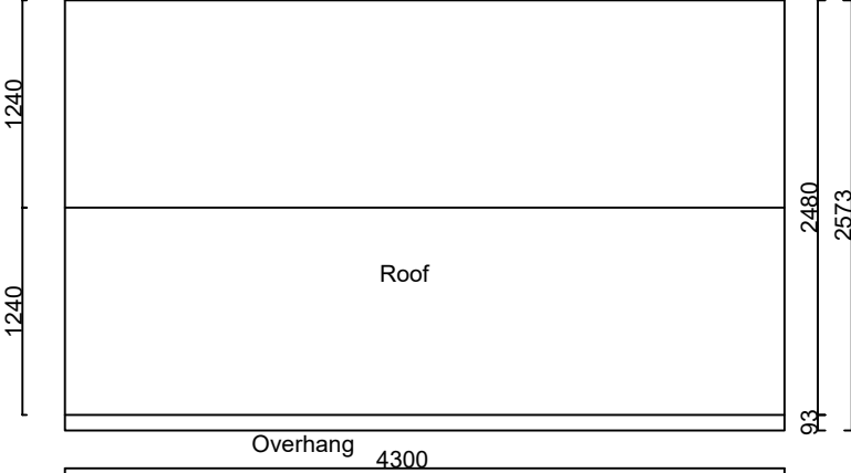
Proposed Roof Layout (1:50)
