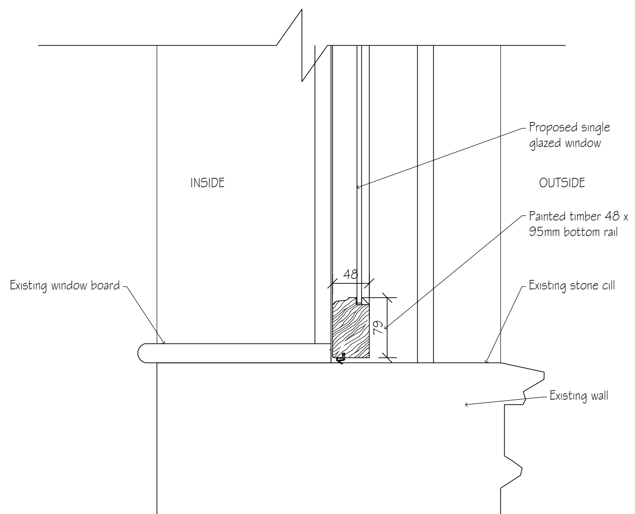
WF06 SECTION 1:5
