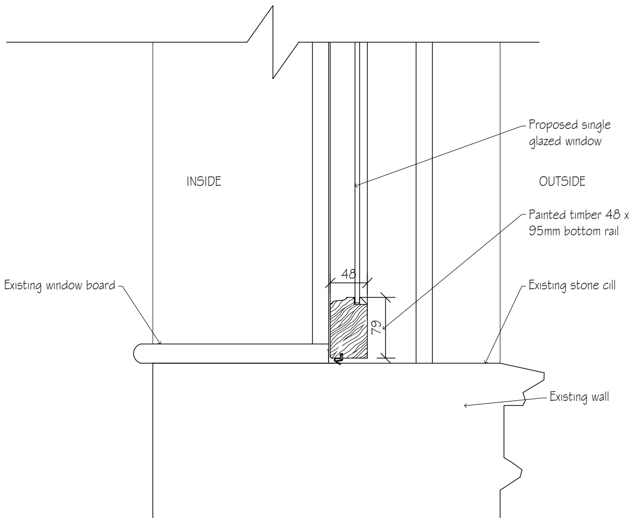
WF05 SECTION 1:5
