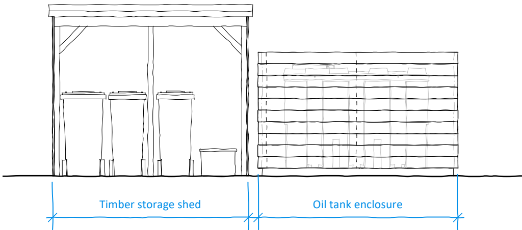
1:50 - Proposed East elevation
