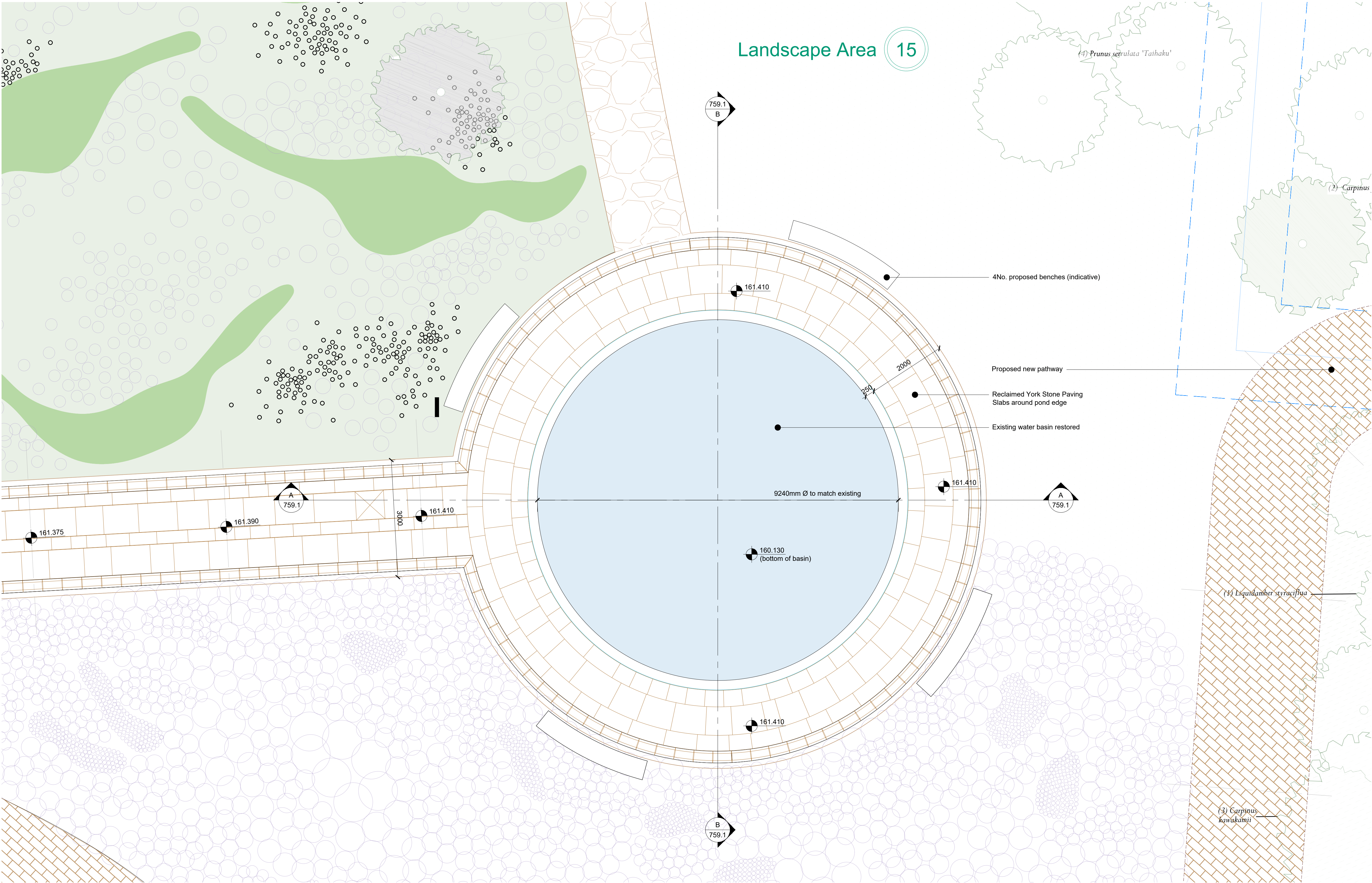
01 Proposed basin (fishpond) - plan 1:50 @_A1
