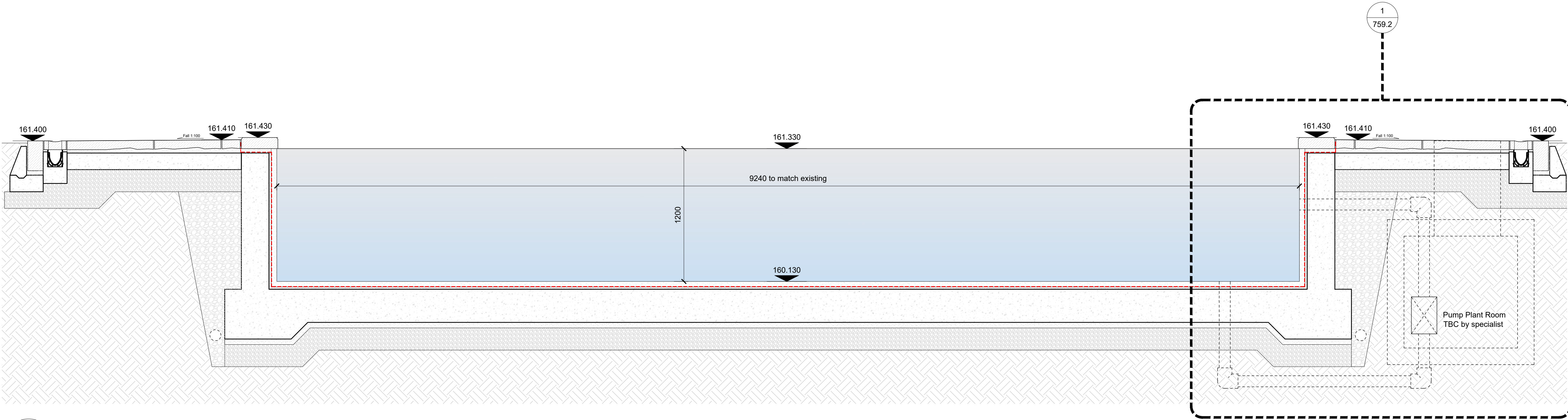
02 Proposed basin (fishpond) - Section B-B 1:20 @_A1
