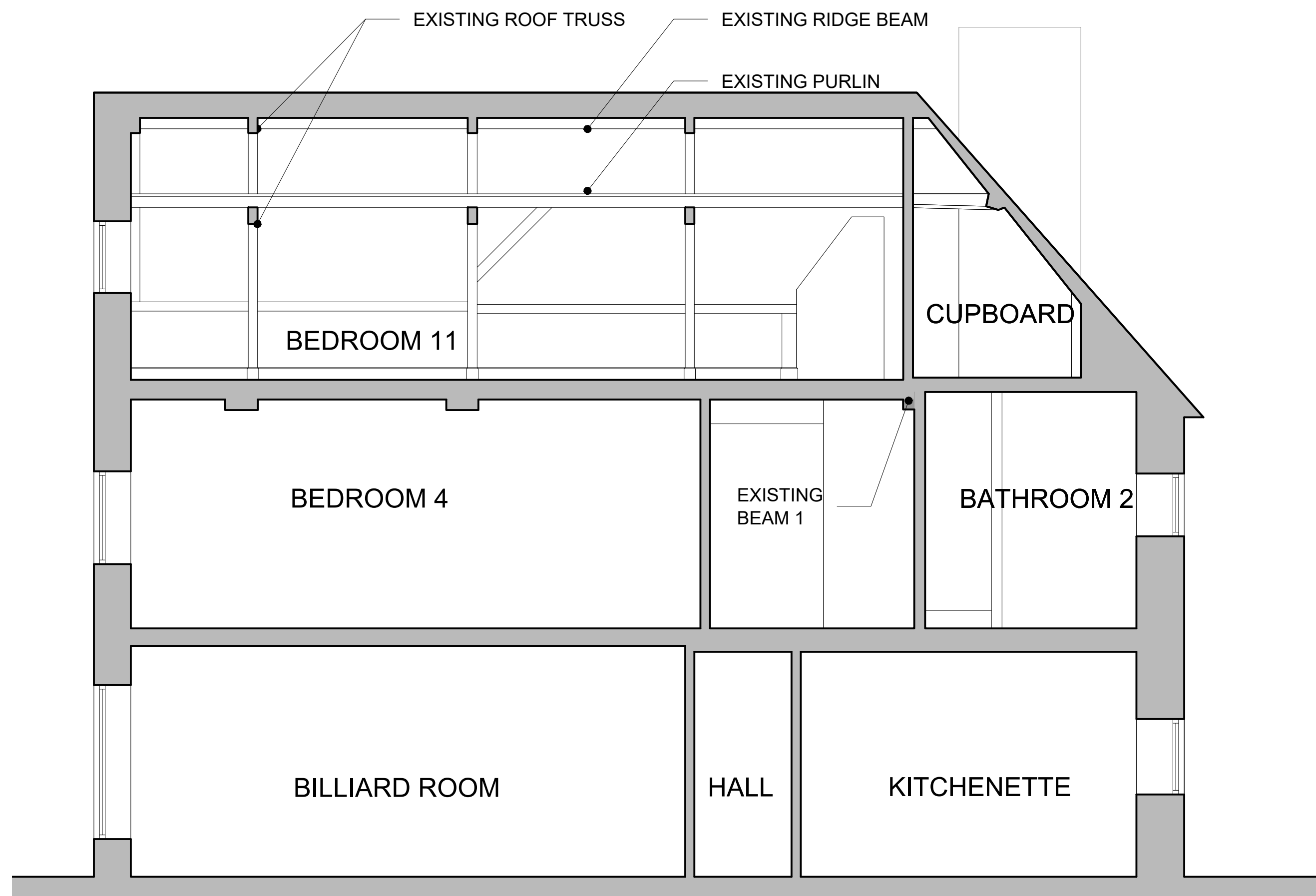
EXISTING SECTION 1-1 Scale 1:50 0 1m 2m 3m Scale bar (1:50)
