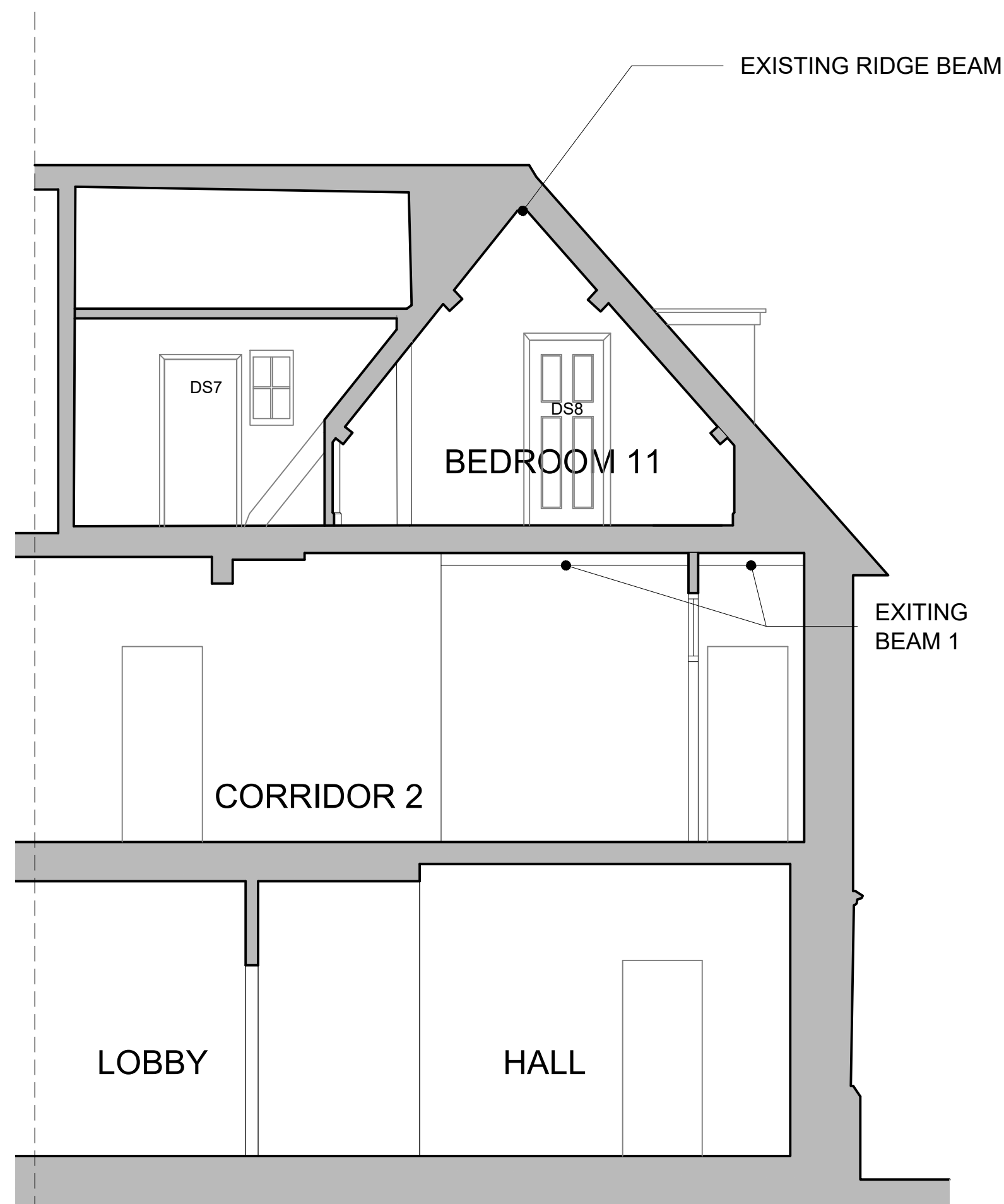
EXISTING SECTION A-A Scale 1:50 0 1m 2m 3m Scale bar (1:50)
