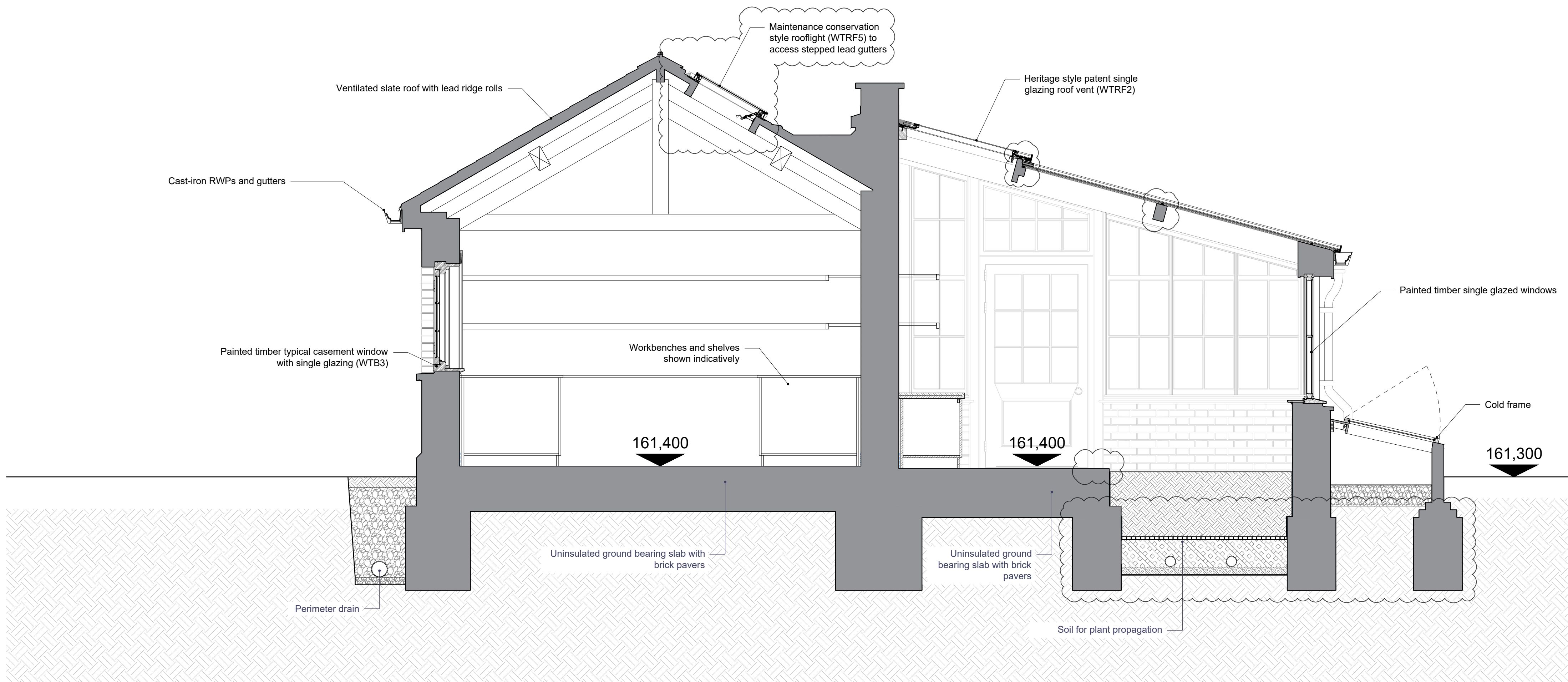
265 Buildings 18 & 19 - Proposed Section A-A 1:25_@_A1
