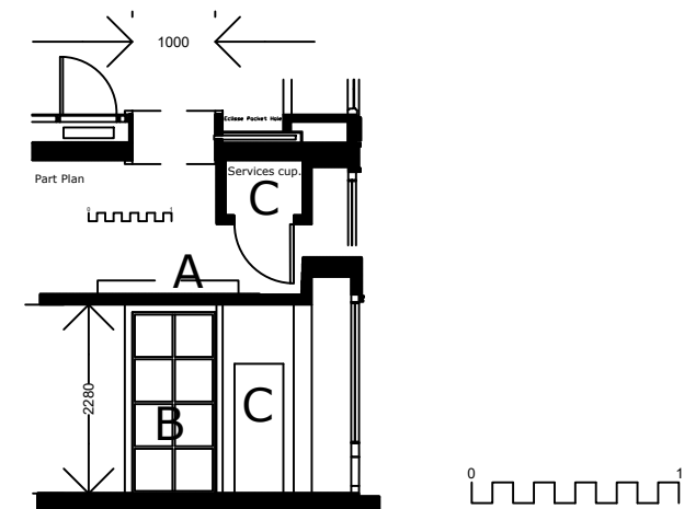
Existing North Elevation
