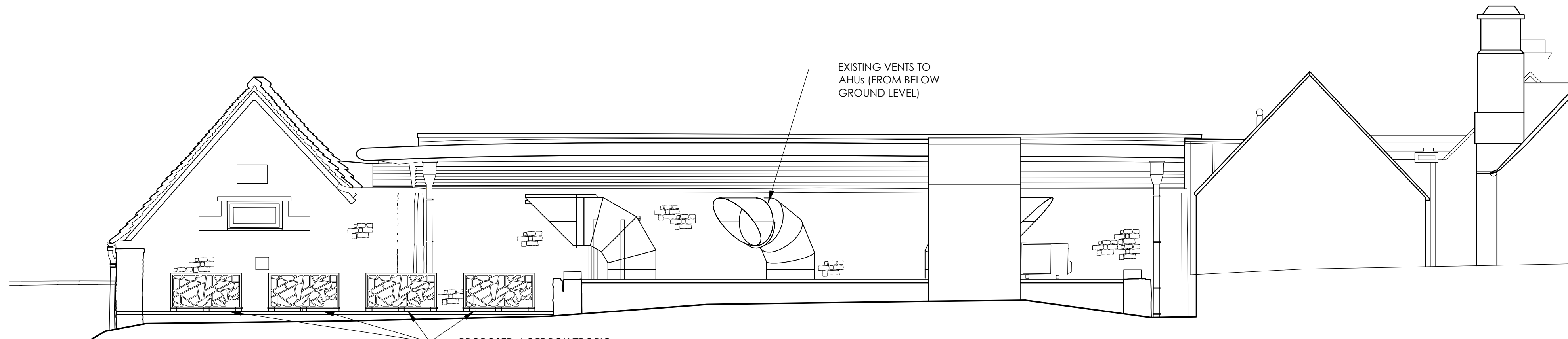
PROPOSED ELEVATION B SCALE 1:50
