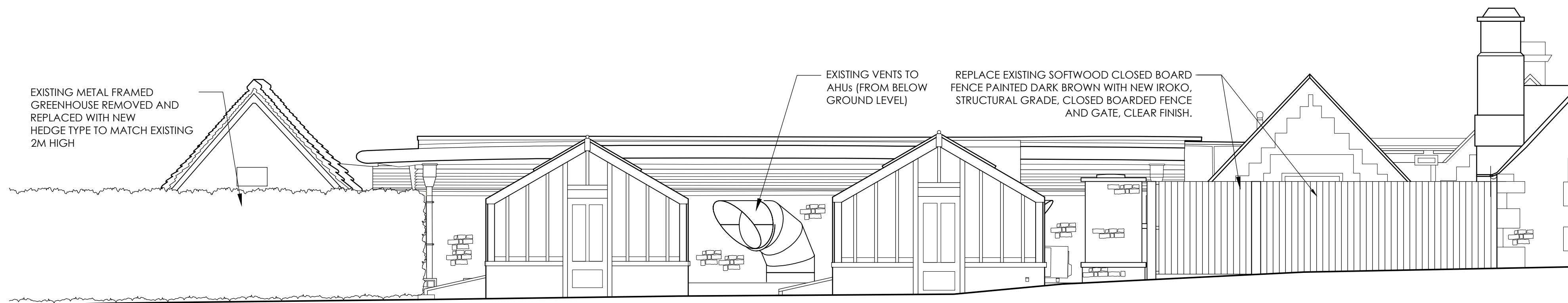
PROPOSED ELEVATION A SCALE 1:50
