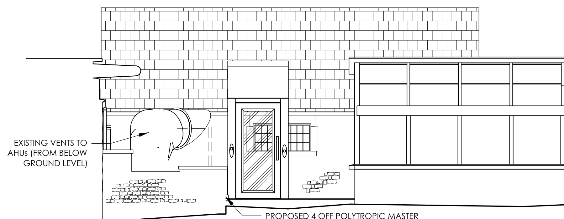
PROPOSED ELEVATION C SCALE 1:50
