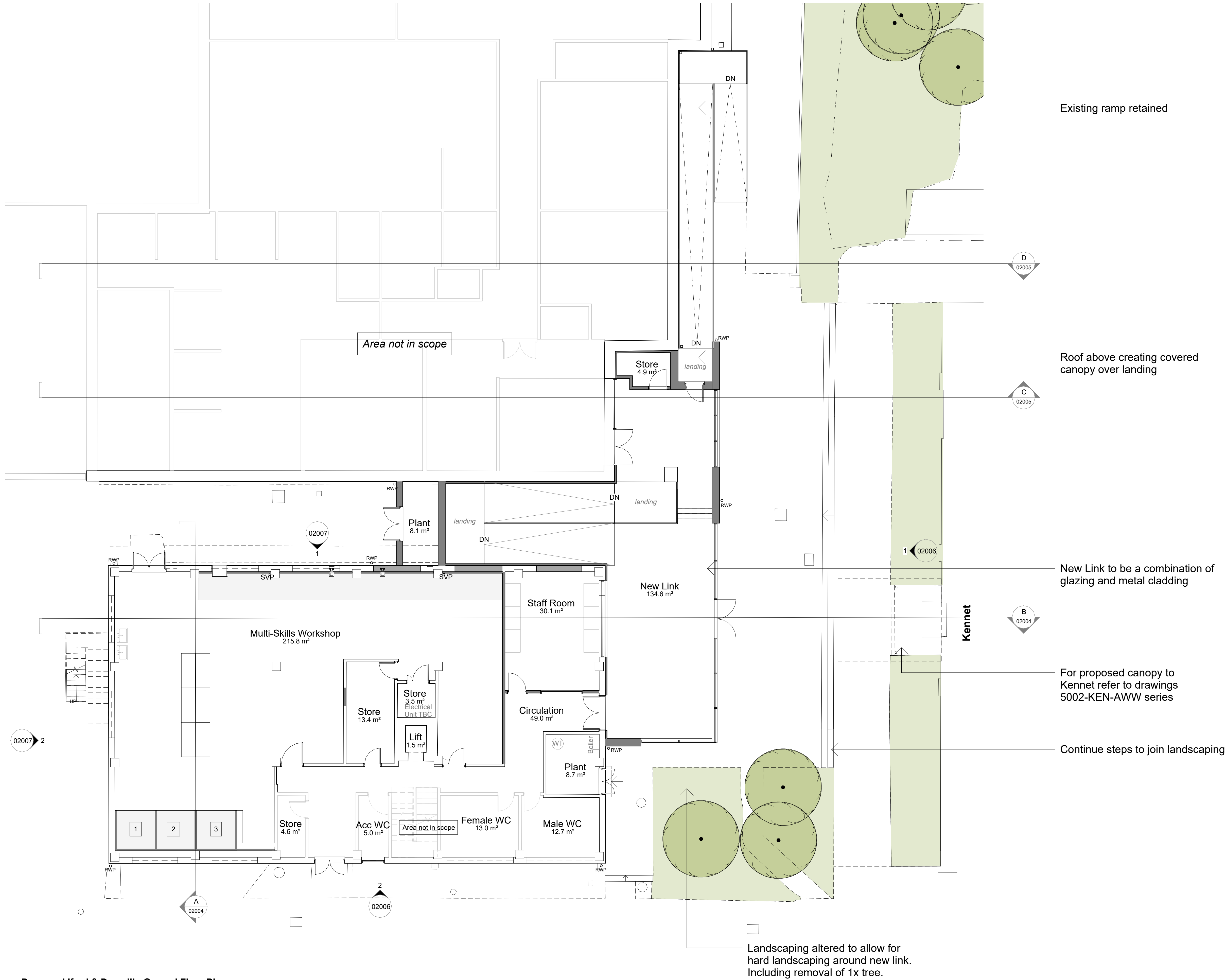
Proposed Iford & Deverill - Ground Floor Plan 1 : 100
